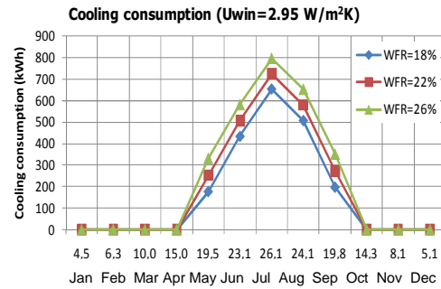
Figure 3. Impact of WFR ratio on the monthly cooling demand, with indication of monthly correspondent T_{sol-air} temperature
