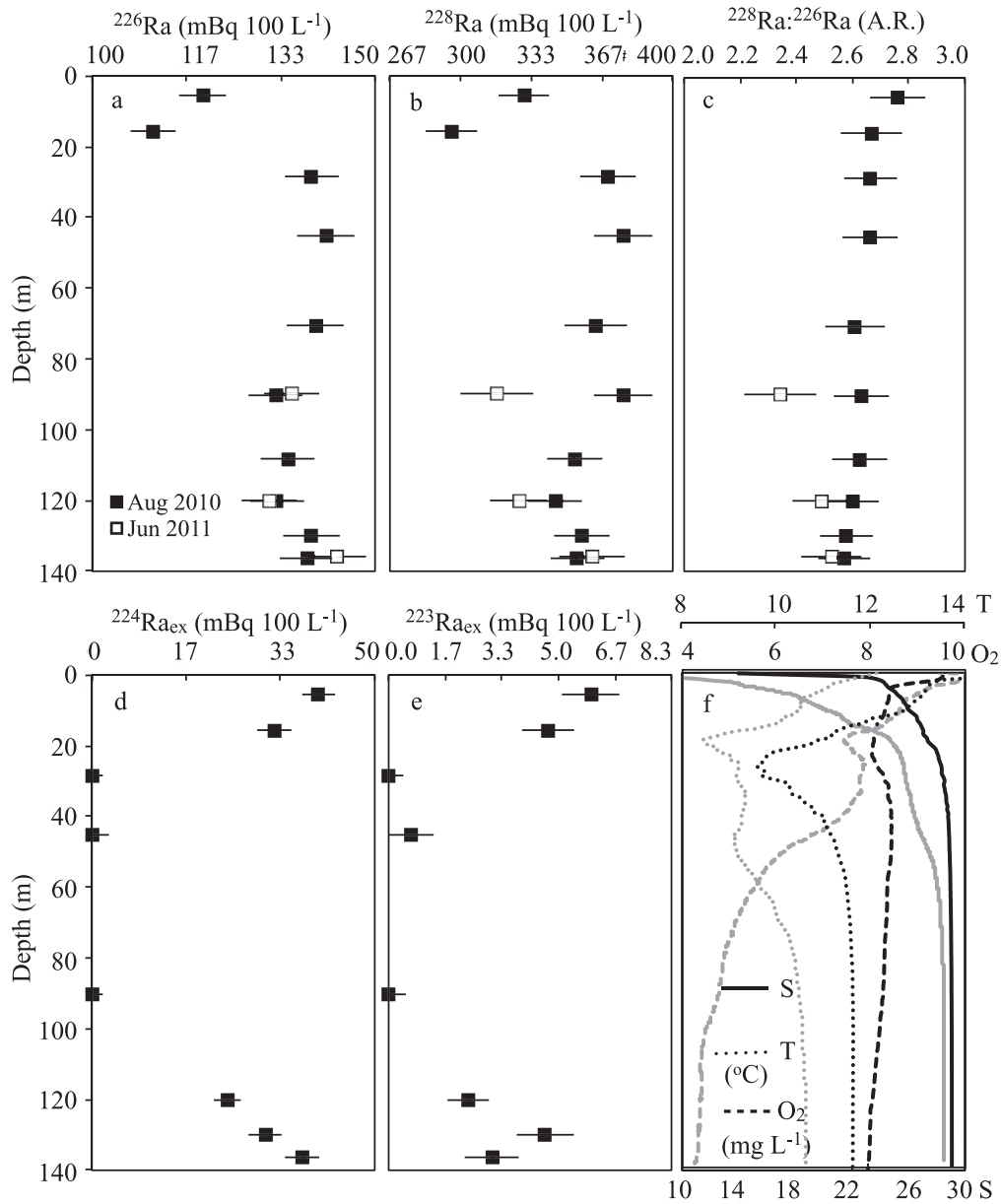
Fig. 4. Water-column profiles of (a) ^{226}\text{Ra} , (b) ^{228}\text{Ra} , (c) ^{228}\text{Ra}:^{226}\text{Ra} , (d) ^{224}\text{Ra}_{\text{ex}} , (e) ^{223}\text{Ra}_{\text{ex}} (mBq 100 L -1 ), and (f) salinity, temperature, and oxygen in the inner basin of Loch Etive. Data are from Sta. LE6, with the black line and filled squares representing data from 03 August 2010 and the gray line and open squares representing data from 08 June 2011. A. R. indicates activity ratio.
