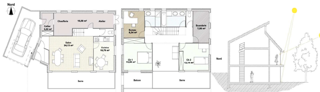
Fig. 1: Zero Energy Building plans (ground floor, first floor and lateral view)
