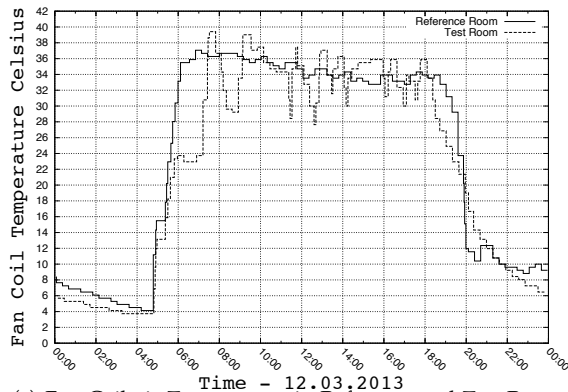
(c) Fan Coil air Temperature in Reference and Test Room
