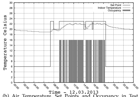
(b) Air Temperature, Set Points and Occupancy in Test Room
