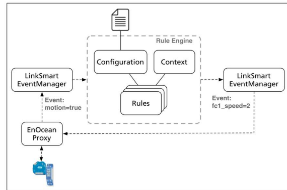
Fig. 6. Rule Engine
