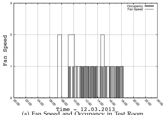
(a) Fan Speed and Occupancy in Test Room
