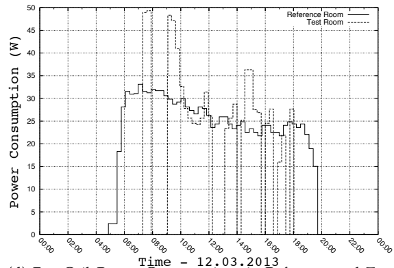
(d) Fan Coil Power Consumptions in Reference and Test Room
