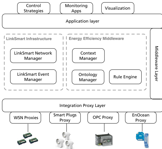
Fig. 1. Software Infrastructure
