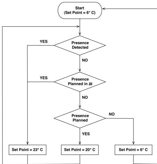
Fig. 7. HVAC Control Strategy
