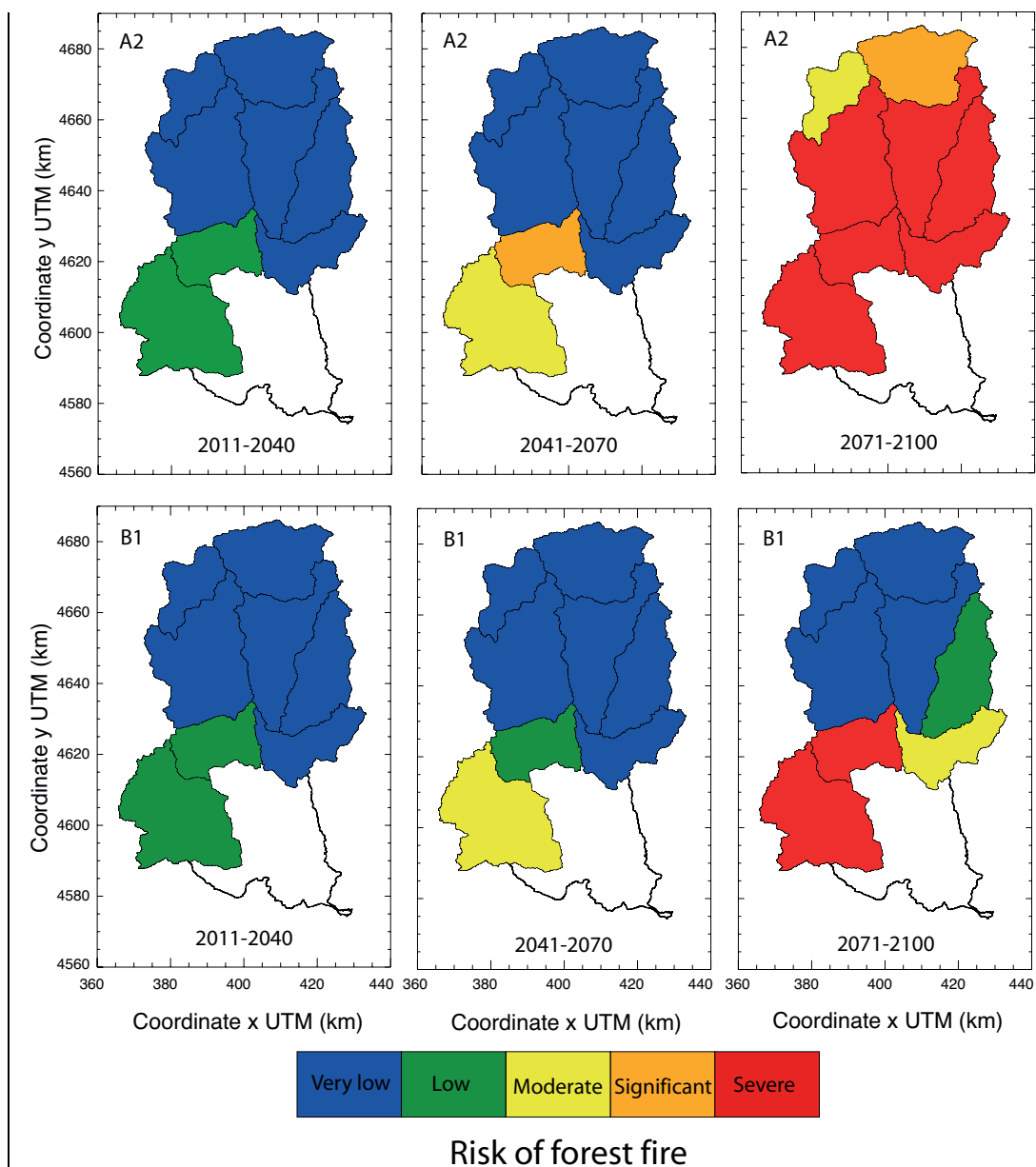
Figure 7. Future scenarios of risk of forest fire for the Llobregat basin based on SMC climate scenarios A2 (top) and B1 (down) for three time periods (2011-2040, 2041-2070, and 2071-2100).
