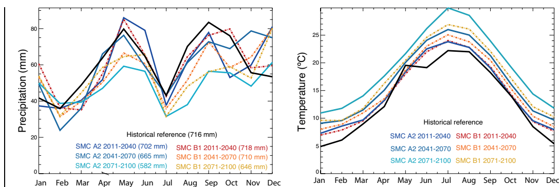
Figure 6. Seasonal precipitation (left) and temperature (right) cycle on the future time period for SMC scenarios (2011-2100). The annual accumulation of precipitation is written in parenthesis.
