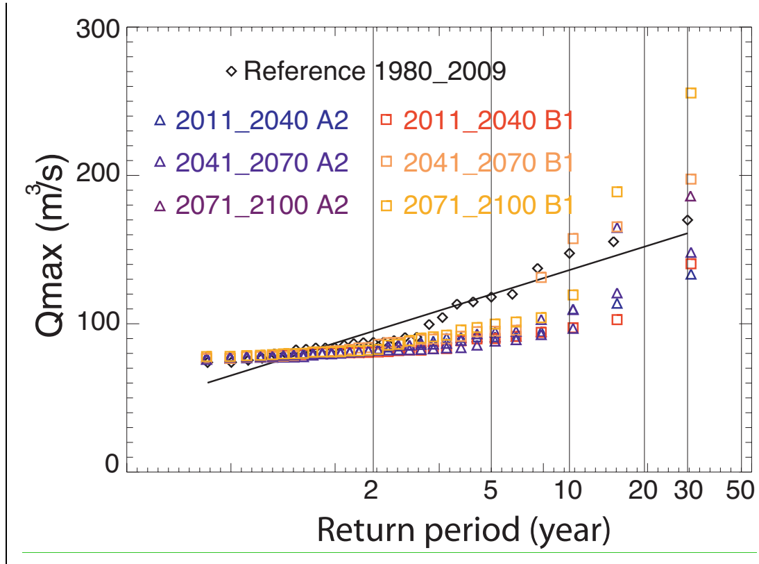
Figure 8. Gumbel distributions of the maximum peak discharge for the different future climate scenarios and time periods. The historical distribution is also represented as a reference (black line).
