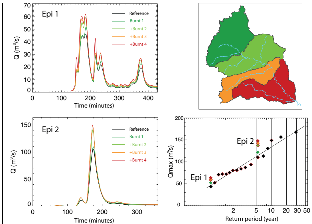
Figure 5. Simulated hydrographs for different situations of burned areas: first the dark green area is burned, then the light green one, then the orange one and finally the red one. The corresponding simulated discharges are represented according to the same colour set for two events. In the bottom right corner, the Gumbel distribution of the maximum discharge is represented: the modified peak discharges are added for the different scenarios of burned area.
