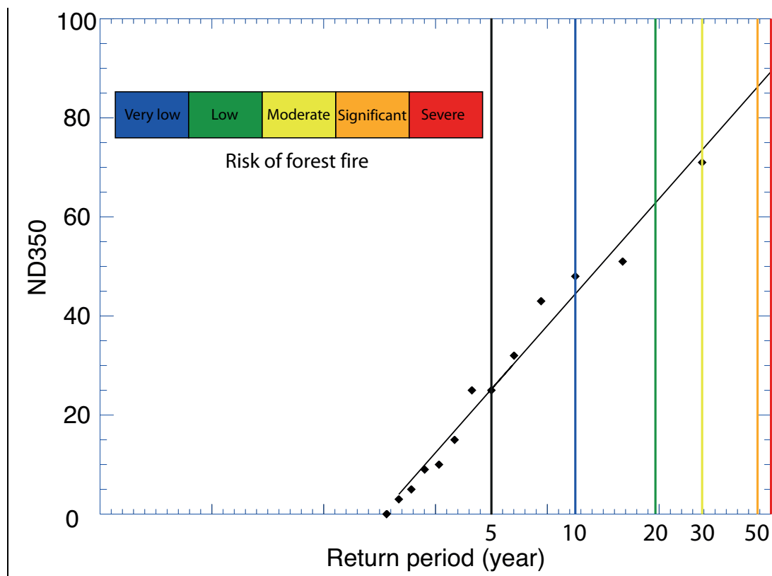
Figure 3. Gumbel distribution adjusted for ND variable representing the number of days per year that exceed the reference threshold of 350 mm. The return periods related to a certain level of risk are added.
