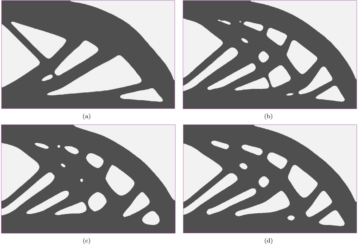
Figure 33: 2d cantilever; optimized shapes for (a): g_{max}^1 = 40 ; (b): g_{max}^1 = 40 and maximum thickness limit d_{max} = 0.40 ; (c): g_{max}^1 = 40 , maximum thickness limit d_{max} = 0.40 and minimum members' distance limit d_{mmd} = 0.05 ; (d): g_{max}^1 = 40 , maximum thickness limit d_{max} = 0.40 and minimum members' distance limit d_{mmd} = 0.10 .
