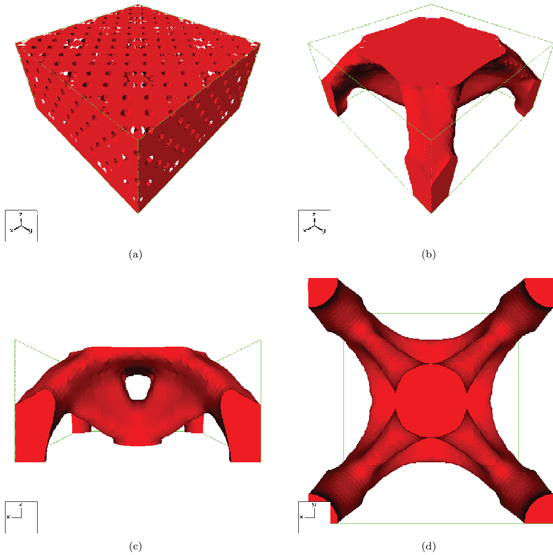
Figure 24: 3d box, using the "approximate" formula; (a): initialization; (b)-(d): different views of the optimized shape for problem (36), g_{max}^1 = 32 and maximum thickness limit d_{max} = 0.60 .
