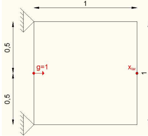
Figure 30: Boundary conditions for the displacement inverter mechanism.
