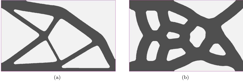
Figure 27: 2d cantilever; optimized shapes (a): for problem (35) (without thickness constraints) and g_{max}^1 = 60 ; (b): for problem (37), g_{max}^1 = 60 and minimum thickness limit d_{min} = 30 imposed since the beginning of the optimization algorithm.
