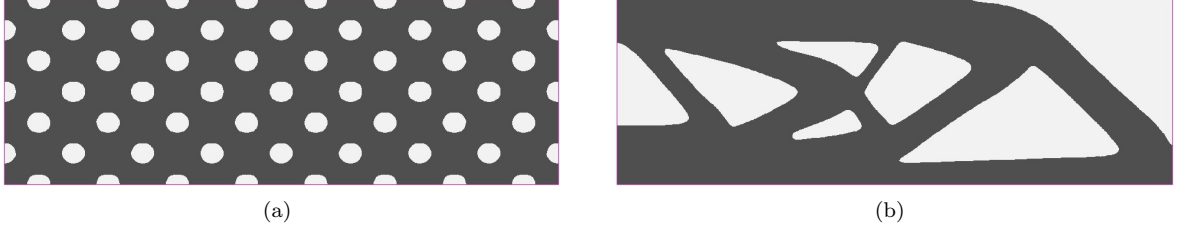
Figure 19: 2d MBB beam; (a): initialization; (b): optimized shape, for problem (35) (no thickness constraint) and g_{max}^1 = 40 .
