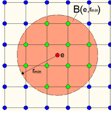
Figure 35: Influence area of an element e .
