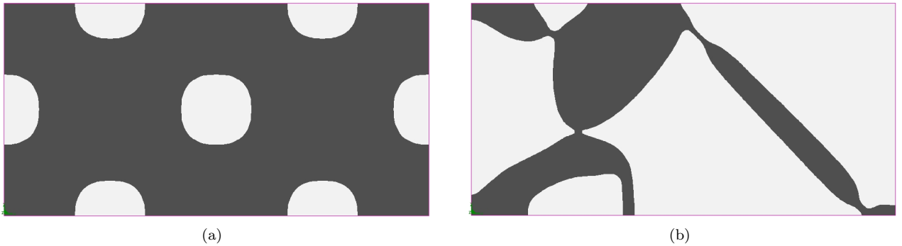
Figure 31: (a): Initialization and (b): optimized shape, without thickness limitations, for the displacement inverter mechanism.
