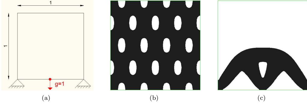
Figure 13: 2d arch; (a): boundary conditions; (b): initialization; (c): optimized shape for the optimization problem (35).
