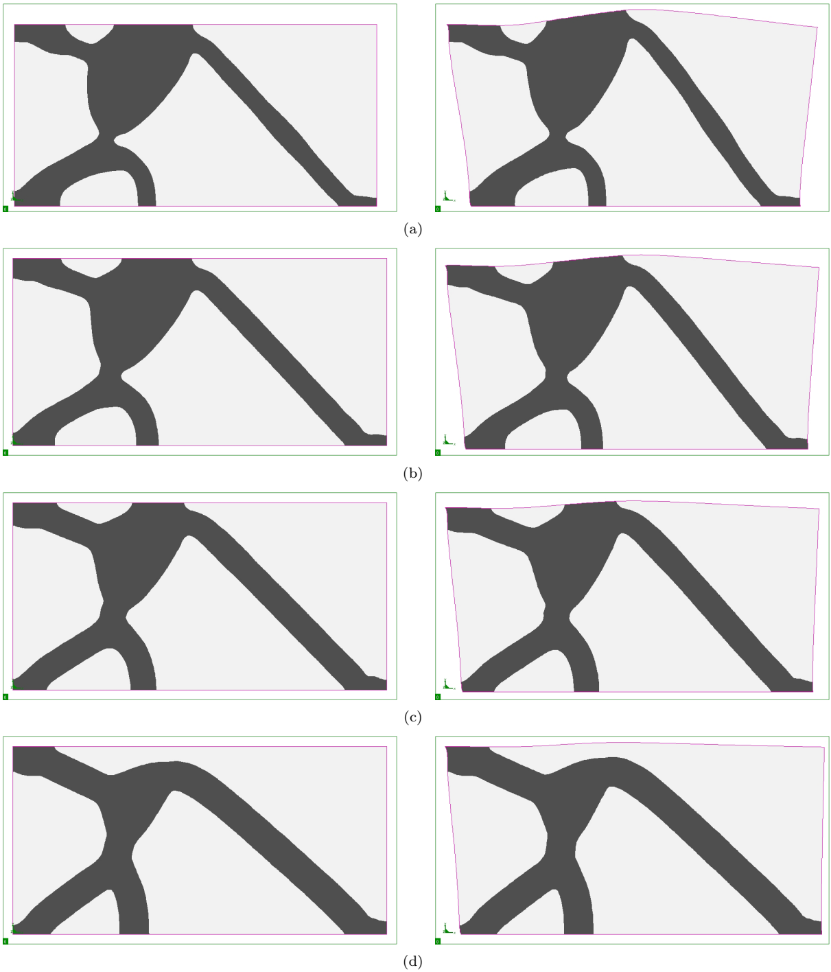
Figure 32: 2d displacement inverter; optimized shapes and deformed configurations imposing a minimum thickness limit (a): d_{min} = 0.05 ; (b): d_{min} = 0.06 ; (c): d_{min} = 0.07 ; (d): d_{min} = 0.08 . The boundary of the working domain D is shown in magenta. A fixed frame is plotted in green to facilitate the comparison of the deformed shapes.
