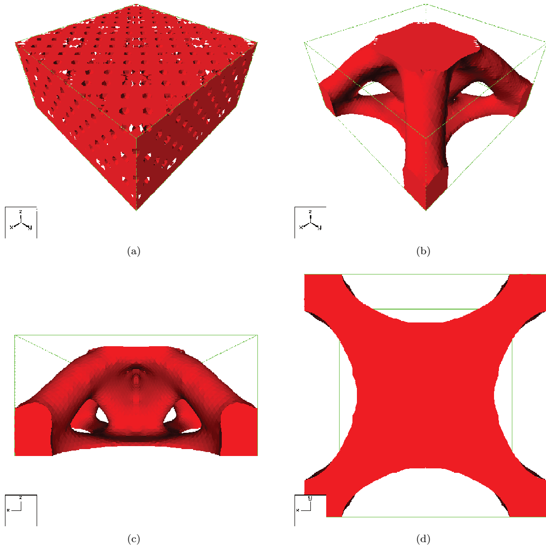
Figure 23: 3d box; (a): initialization; (b)-(d): different views of the optimized shape for problem (35) (without thickness constraints) and g_{max}^1 = 32 .
