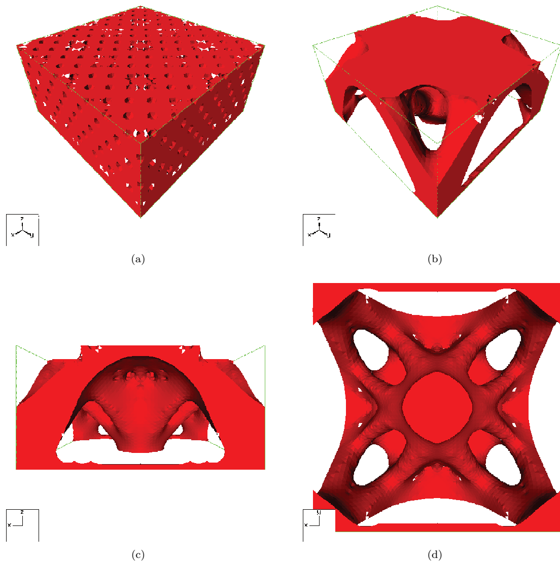
Figure 25: 3d box, using the "approximate" formula; (a): initialization; (b)-(d): different views of the optimized shape for problem (36), g_{max}^1 = 32 and maximum thickness limit d_{max} = 0.40 .
