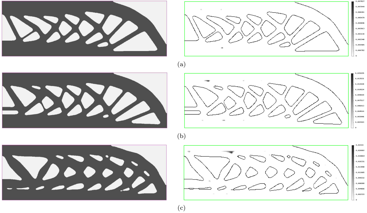
Figure 20: 2d MBB beam, using the "approximate" formula; optimized shapes for problem (36) and maximum thickness violation ( |(d_{\Omega}(x) - d_{max}/2)^-| ) for (a): d_{max} = 0.30 ; (b): d_{max} = 0.25 ; (c): d_{max} = 0.20 .
