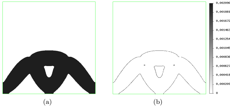
Figure 14: 2d arch using the "true" formula; (a): optimized shape; (b): violation of the constraint |(d_{\Omega}(x) - d_{max}/2)^-| , for the problem (36) and d_{max} = 0.2 .
