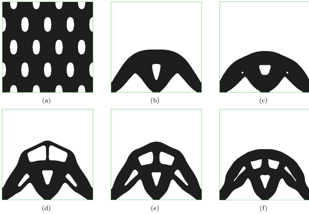
Figure 16: 2d arch; (a): initialization; optimized shapes for the optimization problem (36), using the "approximate" formula (b): without thickness restriction; (c): for d_{max} = 0.20 ; (d): for d_{max} = 0.16 ; (e): for d_{max} = 0.14 ; (f): for d_{max} = 0.12 .
