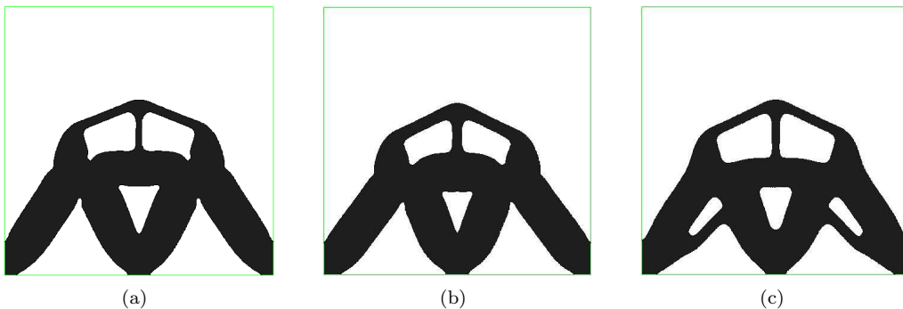
Figure 15: 2d arch; Optimized shapes for problem (36) and d_{max} = 0.16 using the (a): "true"; (b): "Jacobian-free" and (c): "approximate" formulas.
