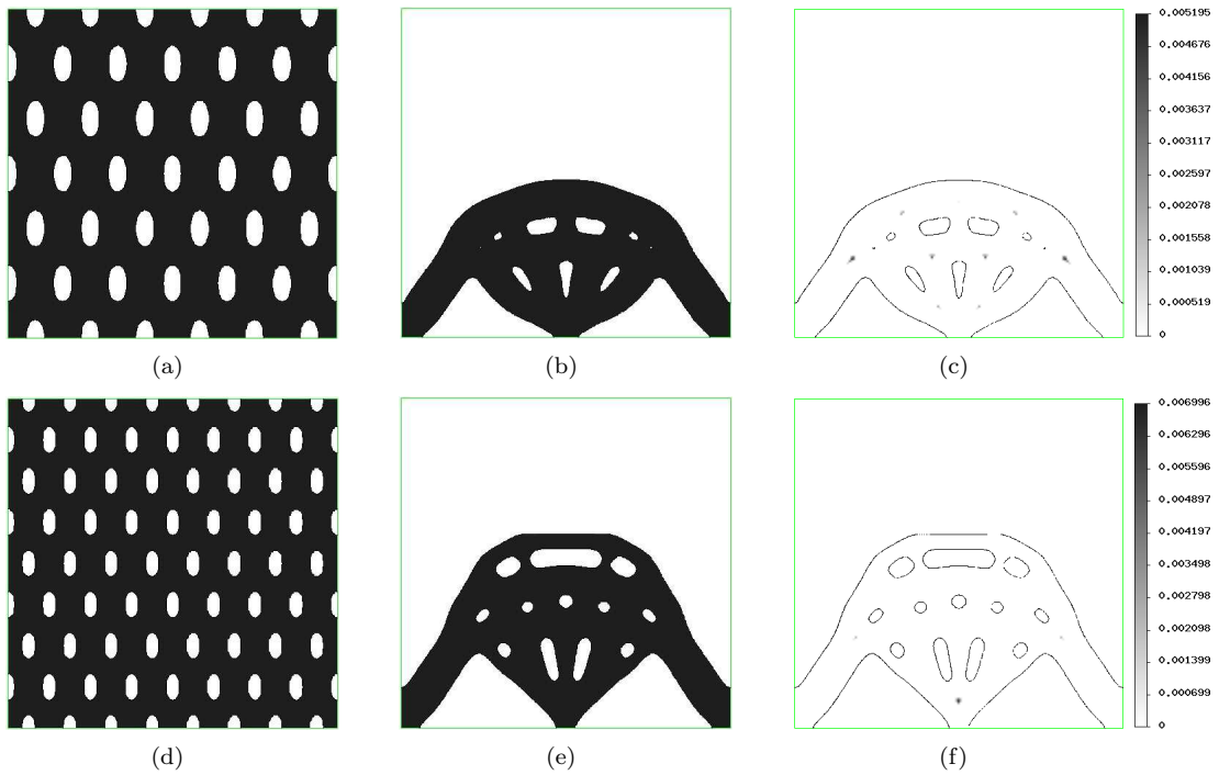
Figure 17: 2d arch using the "approximate" formula; (a),(d): initialization; (b),(e): optimized shape for the optimization problem (36) and d_{max} = 0.12 ; (c),(f): violation of the constraint |(d_{\Omega}(x) - d_{max}/2)^{-}| .
