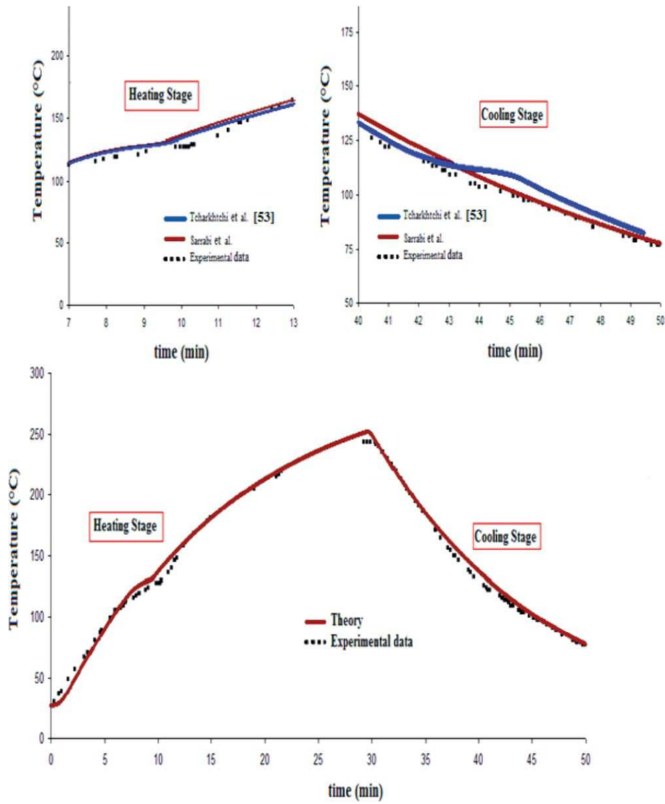
Figure 10. Internal air temperature evolutions for one selected operating conditions. Comparison between experimental and numerical results ( T_{\text{four}} \text{ } \frac{1}{4} \text{ } 300^{\circ}\text{C} , t_c \text{ } \frac{1}{4} \text{ } 30 \text{ min} ). [Color figure can be viewed in the online issue, which is available at wileyonlinelibrary.com.]
