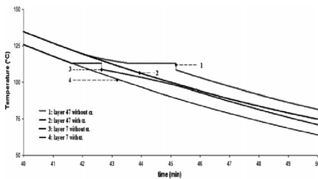
Figure 11. Some “polymer layer” temperature evolutions for one selected operating conditions ( T_{\text{four}} \text{ } \frac{1}{4} \text{ } 300^{\circ}\text{C} , t_c \text{ } \frac{1}{4} \text{ } 30 \text{ min} ). Layer 7 is situated at 40 lm from mold and Layer 47 at 1.6 mm from mold.
