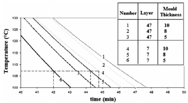
Figure 15. Mold thickness influence (5, 8, and 10 mm) on polymer layer temperature ( T_{four} \approx 300^\circ\text{C} , t_c \approx 30 min).
