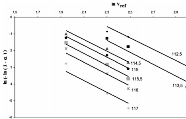
Figure 7. \ln[-\ln(1-a)] versus \ln[V_{ref}] for different temperatures.
