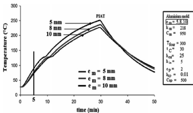
Figure 14. Mold thickness influence (5, 8, and 10 mm) on T-t diagram ( T_{four} \approx 300^\circ\text{C} , t_c \approx 30 min).
