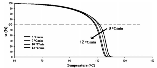
Figure 5. Rate of transformation a versus temperature for different cooling rates ( ^{\circ}\text{C min}^{-1} ).
