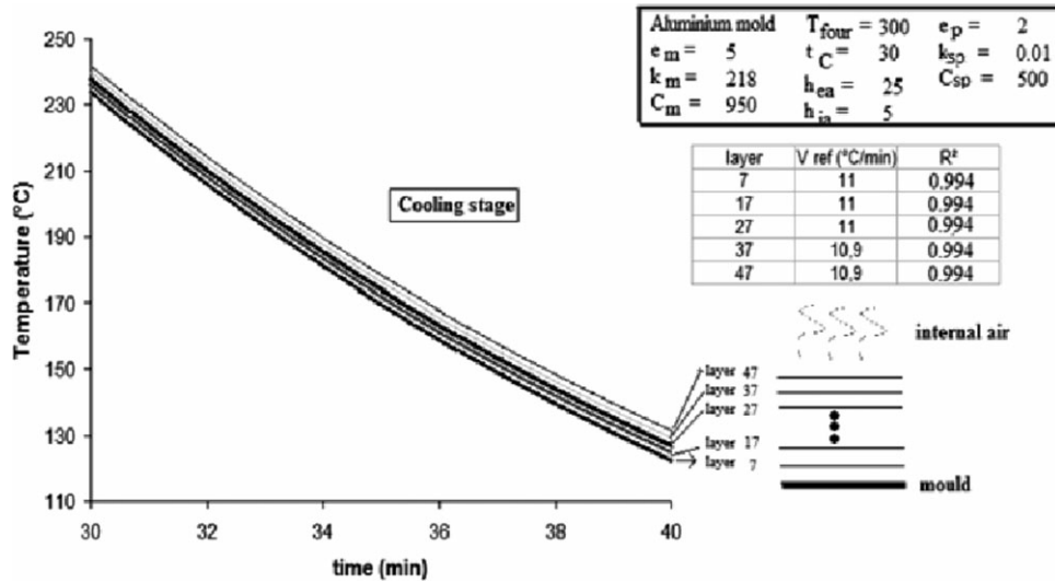
Figure 9. Numerical evolution of temperature from different polymer layers during cooling. Layers 7 (situated at 40 lm from mold) and 47 (situated at 1.6 mm from mold).
