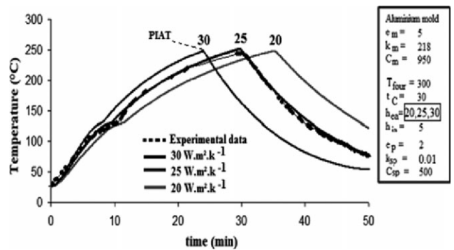
Figure 12. Numerical T-t diagrams obtained with the various coefficients of thermal transfer h_{ca} indicated ( h_{ca} \text{ } \frac{1}{4} \text{ } 20, 25, \text{ and } 30 \text{ W m}^2 \text{ K}^{-1} , T_{four} \text{ } \frac{1}{4} \text{ } 300^{\circ}\text{C} ).
