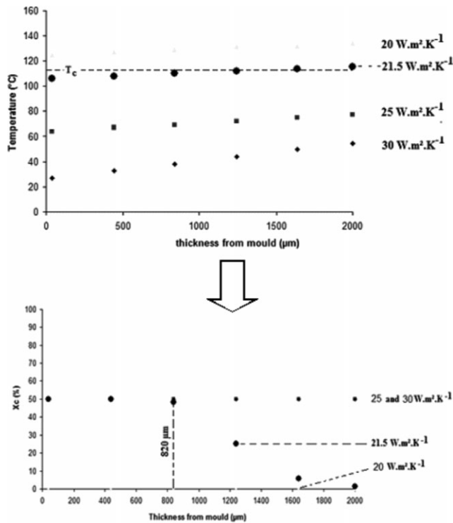
Figure 13. Influence of convection coefficient on temperature (top) and crystallinity ratio (down) of different polymer layers during cooling. h_{ca} \approx 20, 21.5, 25, and 30 \text{ W m}^{-2} \text{ K}^{-1} , T_{four} \approx 300^\circ\text{C} , t_c \approx 30 min, cooling time \approx 20 min).
