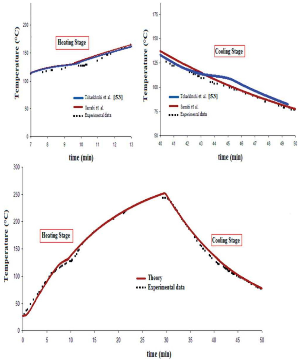
Figure 10. Internal air temperature evolutions for one selected operating conditions. Comparison between experimental and numerical results ( T_{four} \text{ } \frac{1}{4} \text{ } 300^{\circ}\text{C} , t_c \text{ } \frac{1}{4} \text{ } 30 \text{ min} ). [Color figure can be viewed in the online issue, which is available at wileyonlinelibrary.com.]
