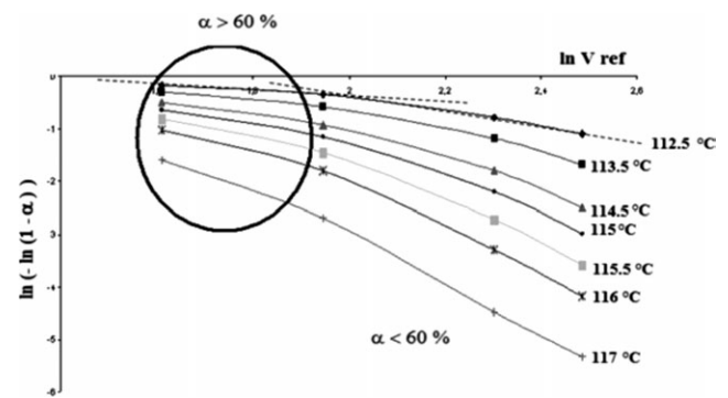
Figure 6. \ln [-\ln (1 - a)] versus \ln [V_{ref}] for different temperatures.
