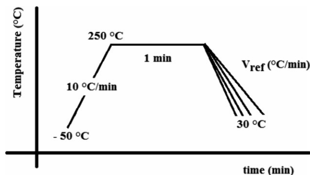
Figure 2. Schematic description of the experimental procedure used in DSC.
