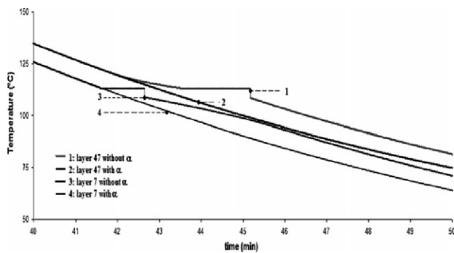
Figure 11. Some “polymer layer” temperature evolutions for one selected operating conditions ( T_{\text{four}} \text{ } \frac{1}{4} \text{ } 300^{\circ}\text{C} , t_c \text{ } \frac{1}{4} \text{ } 30 \text{ min} ). Layer 7 is situated at 40 lm from mold and Layer 47 at 1.6 mm from mold.
