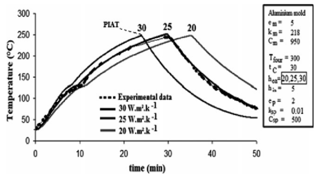
Figure 12. Numerical T-t diagrams obtained with the various coefficients of thermal transfer h_{\text{ea}} indicated ( h_{\text{ea}} \text{ } \frac{1}{4} \text{ } 20, 25, \text{ and } 30 \text{ W m}^2 \text{ K}^{-1} , T_{\text{four}} \text{ } \frac{1}{4} \text{ } 300^{\circ}\text{C} ).
