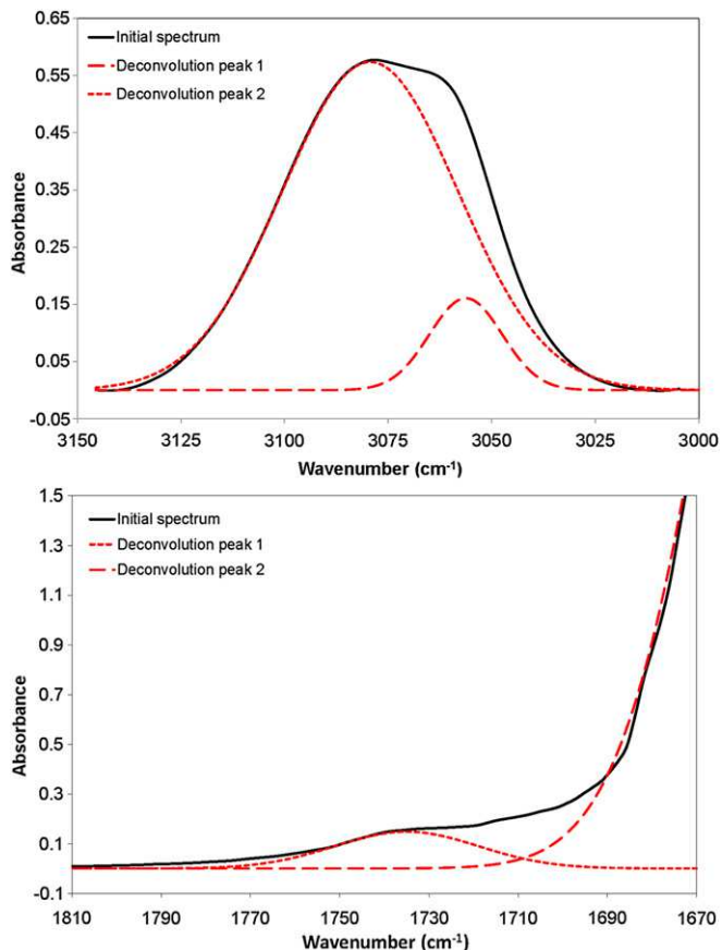
Fig. 5. Mathematical deconvolution of the absorption bands overlapped in the FTIR spectra of a virgin PA 6-6 film (see Fig. 5). Top: Between 3000 and 3150 \text{cm}^{-1} before thermal aging. Bottom: Between 1670 and 1810 \text{cm}^{-1} .
