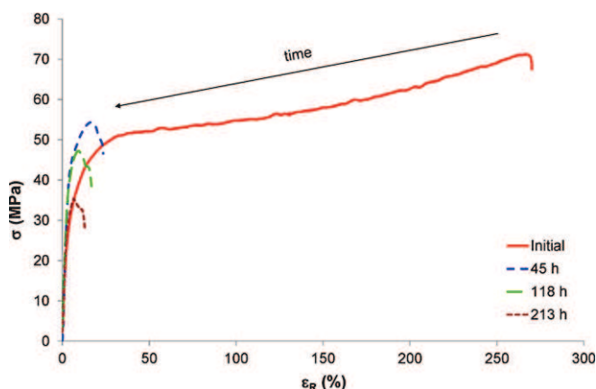
Fig. 8. Tensile curves of PA 6-6 films of about 100 μm thick before and after thermal aging at 100 °C in air.
