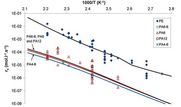
Fig. 10. Arrhenius plot of the maximal oxidation rate ( r_s ) of additive free aliphatic PAs and PE in air or pure oxygen (under atmospheric pressure) between 90 and 200 °C. Comparison between theory (solid lines) and experiment (symbols).
