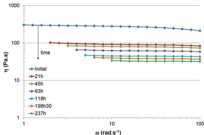
Fig. 7. Curves of dynamic melt viscosity versus angular frequency at 265 °C for PA 6-6 before and after thermal aging at 100 °C in air.
