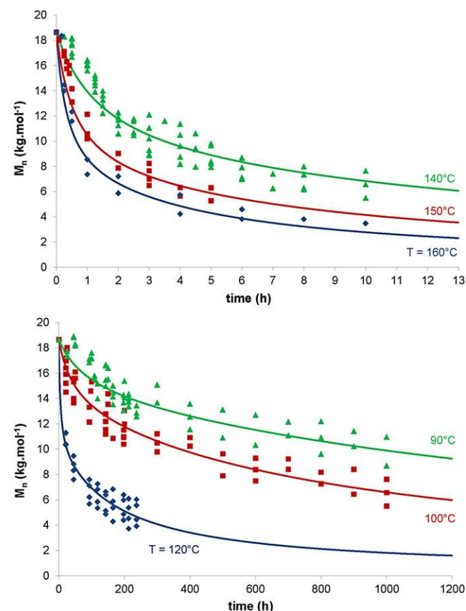
Fig. 11. Changes against time of exposure in the number average molar mass in air between 90 and 160 °C. Comparison between theory (solid lines) and experiment (symbols).
