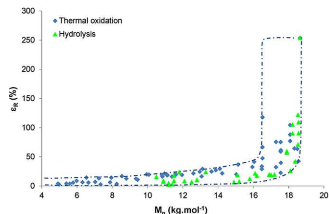
Fig. 12. Ultimate elongation versus number average molar mass for PA 6-6 films of about 100 \mu\text{m} thick exposed in air between 90 and 160 °C or immersed in pure water between 60 and 90 °C.
