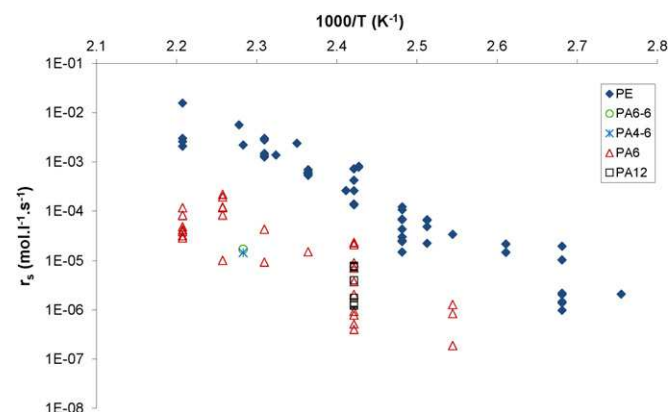
Fig. 2. Arrhenius plot of the maximal oxidation rate ( r_s ) of additive free aliphatic PAs and PE in air or pure oxygen (under atmospheric pressure) between 90 and 200 °C.
