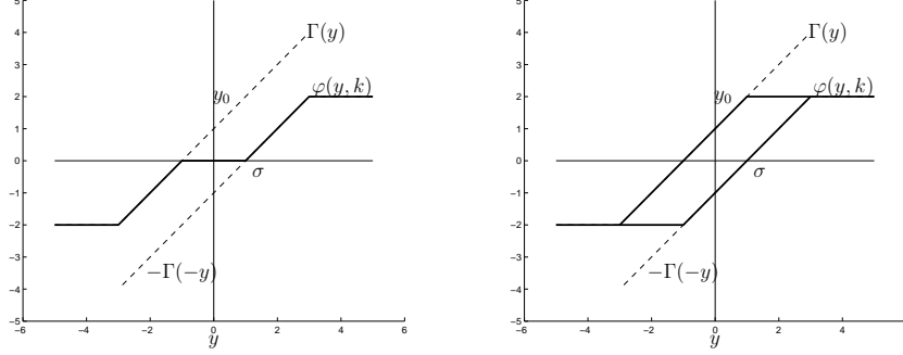
Figure 1: Examples: saturation plus dead-zone ( left ) and hysteresis ( right ).
