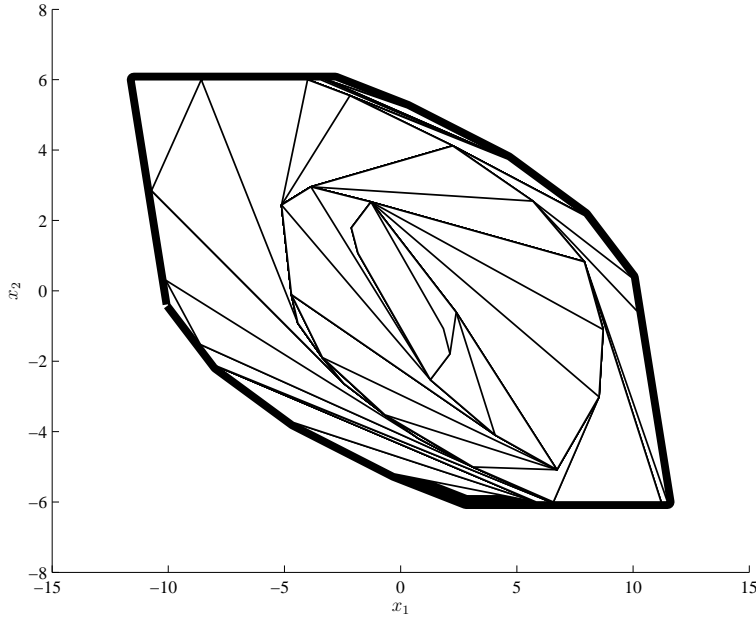
Figure 2: Sequence of sets \Omega_k for the CDI system, for k \in \mathbb{N}_{[0, k_{max}]} , generated by Algorithm 1.
