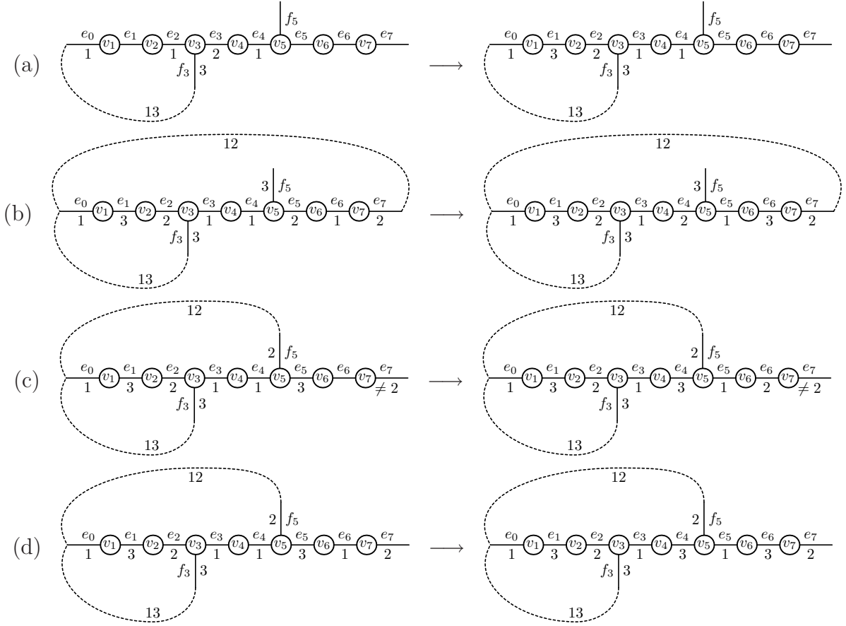
Figure 7: Reducing a path with degrees 2, 2, 3, 2, 3, 2, 2.
