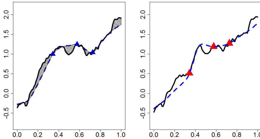
Fig. 2 Left: kriging residual r^{(i)} = z^{(i)} - m_q^{(i)} obtained by non-conditional simulation of a replicate Z^{(i)} of a non-stationary GRF Z (black solid line) and its simple kriging mean (blue dashed line) based on q = 3 observations (blue triangles) at a design \mathbf{X}_q . Right: conditional simulation of Z (solid black line) obtained by summing Z 's simple kriging mean (blue dashed line) based on its values at the same design \mathbf{X}_q (red triangles) and the kriging residual r^{(i)} simulated on the left graph.
