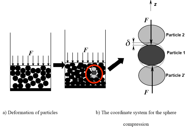
Figure 5: Principle of the Hertz model.
