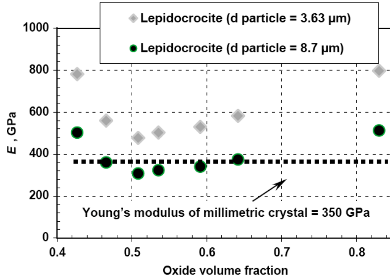
Figure 6: Young modulus derived from the Hertz theory.
