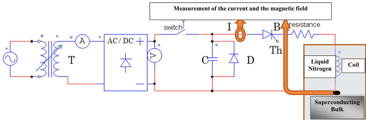
Figure 4. Electrical circuit.
