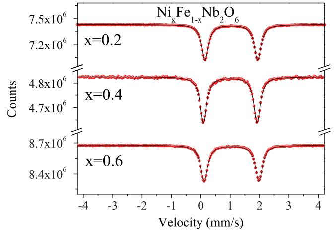
FIG. 10. (Color online) ^{57}\text{Fe} Mössbauer spectra recorded at room temperature on the indicated compounds of the \text{Ni}_x\text{Fe}_{1-x}\text{Nb}_2\text{O}_6 series. The points are the experimental data and the line is the corresponding fitting.
