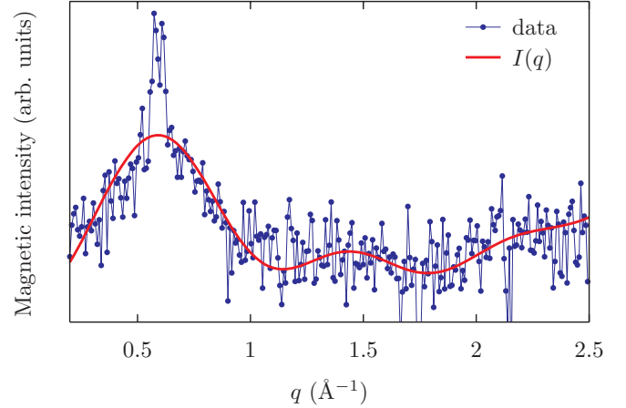
FIG. 5. (Color online) Detailed view of the diffuse neutron scattering pattern for \text{Ni}_{0.8}\text{Fe}_{0.2}\text{Nb}_2\text{O}_6 . The line is a fitting to Eq. (2). One can see a precursor of a Bragg peak growing on top of the diffuse signal.
