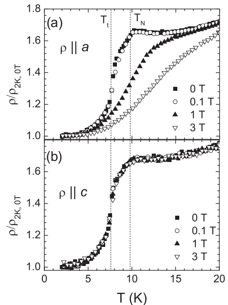
FIG. 2. Relative electrical resistivity and magnetoresistivity of NdRhSn for (a) \rho||a axis, B||c axis and (b) \rho||c axis, B||a axis. The dashed lines represent the positions of T_N and T_t . All data were obtained during the increasing of the temperature.
