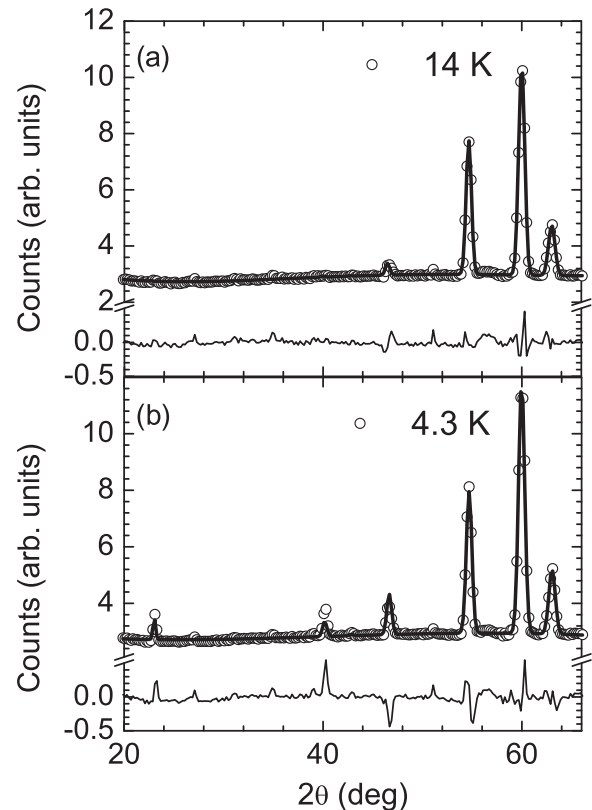
FIG. 4. Representative powder neutron-diffraction patterns of NdRhSn at (a) 14 K and (b) 4.3 K. The circles represents the experimental data, the line through circles represents the best Rietveld fit, and the line below the circles represents the difference.
