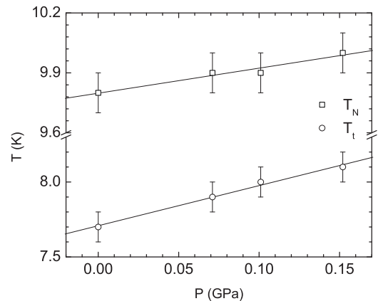
FIG. 10. Evolution of the transition temperatures T_N and T_t of NdRhSn at B = 0.01 \text{ T} under uniaxial pressure. The data have been taken for the experimental configuration B \parallel p \parallel c axis.
