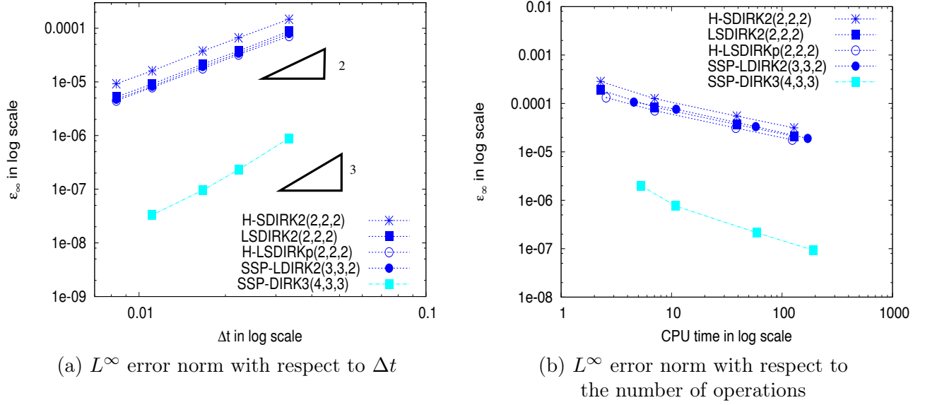
FIGURE 5. Test 2 - Nonlinear convection-diffusion problem: (a) L^\infty error norm for the second order schemes (23), (26), (24), (25) and (27) and the third order SSP- DIRK3(4,3,3) L-stable scheme (28).
