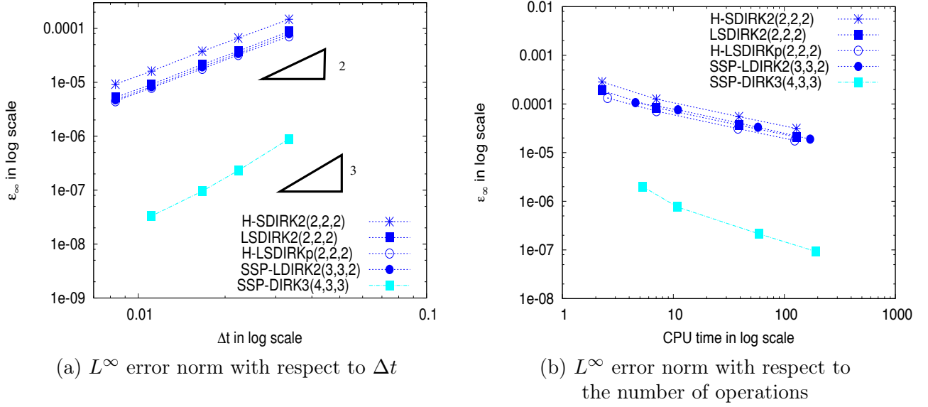
FIGURE 5. Test 2 - Nonlinear convection-diffusion problem: (a) L^\infty error norm for the second order schemes (23), (26), (24), (25) and (27) and the third order SSP- DIRK3(4,3,3) L-stable scheme (28).
