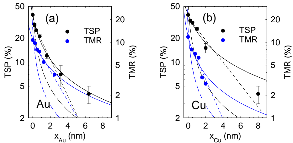
Figure 6. (Colour online) Transport properties of junctions doped at the Co/ \text{AlO}_x interface with (a) Au and (b) Cu. The TSP is plotted on the left-hand ordinate in each graph, the TMR on the right-hand one. The dotted lines are fits of an exponential decay to the data, which appear as straight lines on these semi-log plots. The dashed lines are a fit of the model described in reference [32] with a = 0.223 nm, the value for the atomic size of Co. The solid lines are fits with a as a variable parameter. (The data, but not the analysis, in panel (a) were previously shown in reference [31].)
