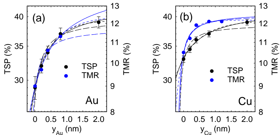
Figure 7. Transport properties of junctions \delta -doped within the Co electrode with (a) Au, and (b) Cu. The TSP is plotted on the left-hand ordinate in each graph, the TMR on the right-hand one. The dotted lines are fits of an exponential rise to the data. The dashed lines are a fit of the model described in reference [32] with the modifications described in the text, with b set to the value for the atomic size for Au ( b = 0.257 nm) or Cu ( b = 0.227 nm). The solid lines are fits with b as a variable parameter. (The data, but not the analysis, in panel (a) were previously shown in reference [31].)
