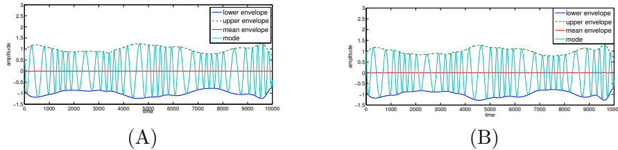
Figure 4: The signal m^f obtained from the signal x of Figure 3.(A) as well as its upper and lower envelopes, for one interval strategy (A) and for three intervals strategy (B).
