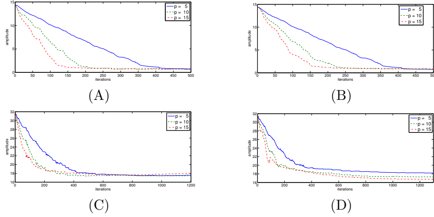
Figure 5: L^2 norm of m^j with respect to j , for one interval strategy (A) and for three intervals strategy (B). (C) and (D): L^2 error of x_1 - m^j with respect to j , for one interval strategy (C) and for three intervals strategy (D).
