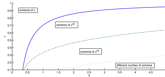
Figure 2. Different regions for the best approximations of \theta by t, t^{(2)}, t^{(4)}
