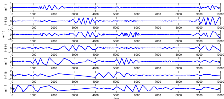
Figure 1: Some of the significant mode obtained for the decomposition of the signal of Figure 3.(A)
