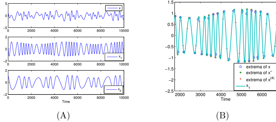
Figure 3: (A): signal x made of two modulated signals x_1 and x_2 . (B): signal x_1 and its values at t , t^{(2)} and t^{(4)} .
