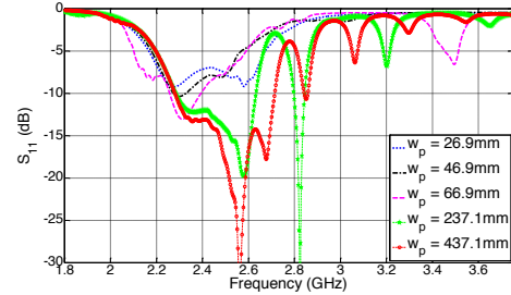
Figure 4. Simulated reflection coefficients of the HIS based dipole antenna for different patch width values.
