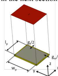
Figure 1. Phase reflection simulation of the patch unit-cell.
