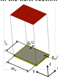
Figure 1. Phase reflection simulation of the patch unit-cell.
