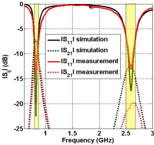
Figure 2: Simulated and measured S-parameters.
