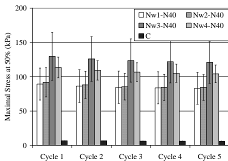
Figure 24. Maximum stress at 50% of initial thickness deformation of laminated samples Nw1-N40 and C
