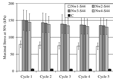
Figure 23. Maximum stress at 50% of initial thickness deformation of laminated samples Nw1-S44 and C
