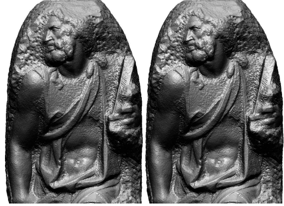
Figure 6: Rendering of the original (left) and decompressed Stanford St Matthew (right), both have 93.4 million points. R = 3mm, N_{bins} = 16
