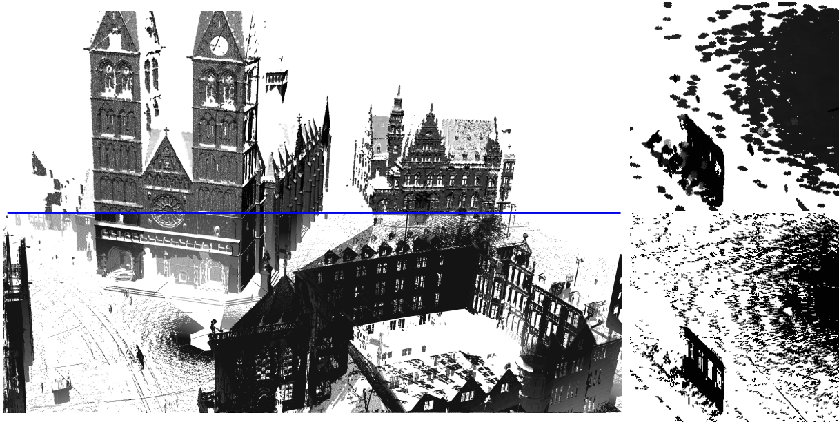
Figure 12: Left : the Bremen point cloud (bottom) and the decompressed result (top). Right : closeup views : original (bottom) and decompressed (top) R = 18\text{cm}, N_{bins} = 16 . In sparsely sampled areas, two phenomena occur: if the sampling is too low, the points are removed during the pre-processing step and if the sampling is above the limit, there is a dilatation effect clearly visible in the closeups (right).
