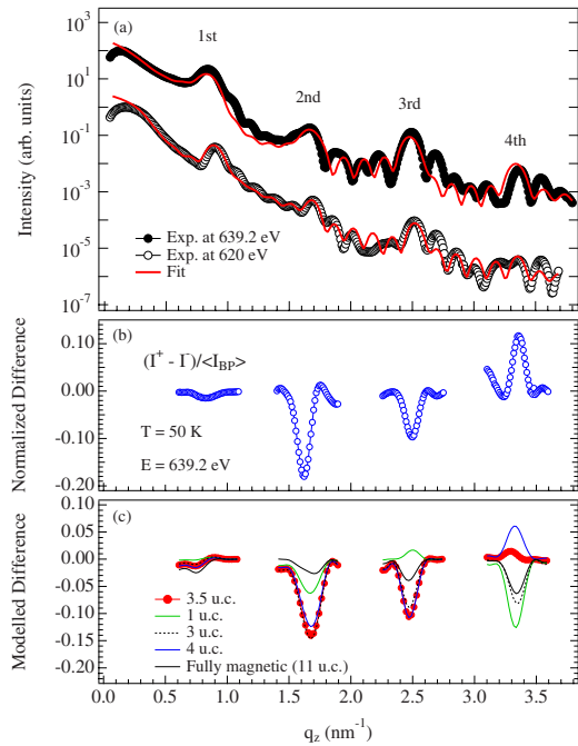
FIG. 7. (Color online) (a) Specular reflectivity measured at 50 K for E=639.2 eV on the Mn L_3 edge (upper trace) and at room temperature with photon energy E=620 eV, below the Mn L_3 edge (lower trace). The lines are the results of fits to a structural model discussed in the text. The Bragg-peak positions are indicated. (b) Dichroic differences I^+ - I^- measured at the Bragg-peak positions, normalized to the peak intensity. (c) Calculated normalized difference at the same Bragg-peak positions for different layer thicknesses of the interface magnetized regions in \text{CaMnO}_3 .
