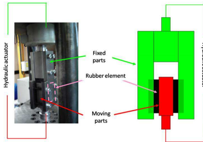
Figure 8. Shear bench
