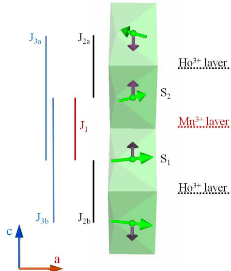
FIG. 6. (Color online) Labeling scheme and relevant interactions for the linear-chain model. Purple (dark grey) arrows represent ionic displacements while green (light grey) arrows represent the spin ordering from reference [11]
