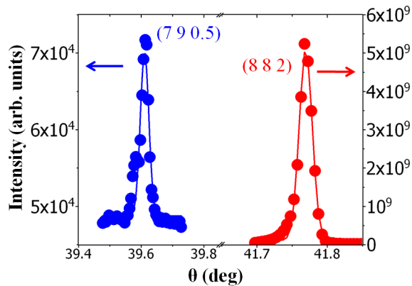
FIG. 1. Peak profiles of the (7 9 0.5) and (8 8 2). The line is a fit to the data with a Lorentian profile function.
