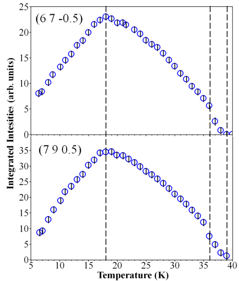
FIG. 2. Temperature dependence of integrated intensities of SL peaks: (6 7 -0.5) (upper panel) and (7 9 0.5) (bottom panel).
