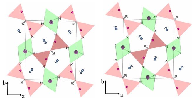
FIG. 4. (Color online) Representation of the observed ionic displacements ( \mathbf{k}_c=(0\ 0\ 0.5) ) in \text{HoMn}_2\text{O}_5 with arrows (magnified by 1000). The structure is shown in one unit-cell, marked by thin black lines, along the a - and b -axis. The projection is separately shown for ionic displacements sites belonging to adjacent crystallographic cells along the c -direction. The purple (small and light grey), grey and blue (black) arrows represent ionic displacements on Mn , O^{2+} and Ho^{3+} sites respectively. Corresponding Mn-O polyhedra are also shown.
