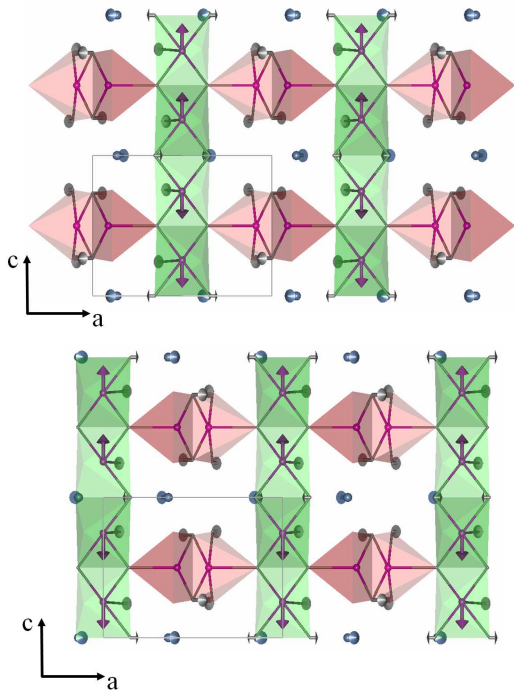
FIG. 5. (Color online) Representation of the observed ionic displacements ( \mathbf{k}_c=(0\ 0\ 0.5) ) in \text{HoMn}_2\text{O}_5 with arrows (magnified by 1000). The structure is shown in four unit-cells, marked by thin black lines (only one cell), along the a - and c -axis. The projection is separately shown for ionic sites belonging to the first zig-zag chain (top) and the second chain (bottom). The purple (small and light grey), grey and blue (black) arrows represent ionic displacements on \text{Mn} , \text{O}^{2+} and \text{Ho}^{3+} sites respectively. The green (light grey) horizontal arrows inside the \text{Mn}^{4+} polyhedra represent the spin ordering of \text{Mn}^{4+} from reference [11]. Corresponding Mn-O polyhedra are also shown.
