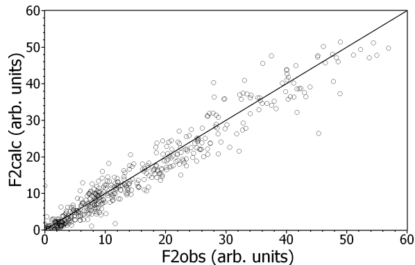
FIG. 3. Results of the refinement with \mathbf{k}_c=(0\ 0\ 0.5) for the ionic displacement for \text{HoMn}_2\text{O}_5 compound. The experimental structure factors are plotted against the calculated ones. The agreement factors are R(F) factors and \chi^2 are 10% and 10.3 respectively.
