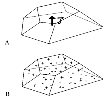
Fig. 1. Example of polyhedron-shaped magnet. (A) Constant and uniform magnetization, \mathbf{J} is the polarization in Tesla.. (B) Equivalent coulombian representation (surface distribution of magnetic charges).
