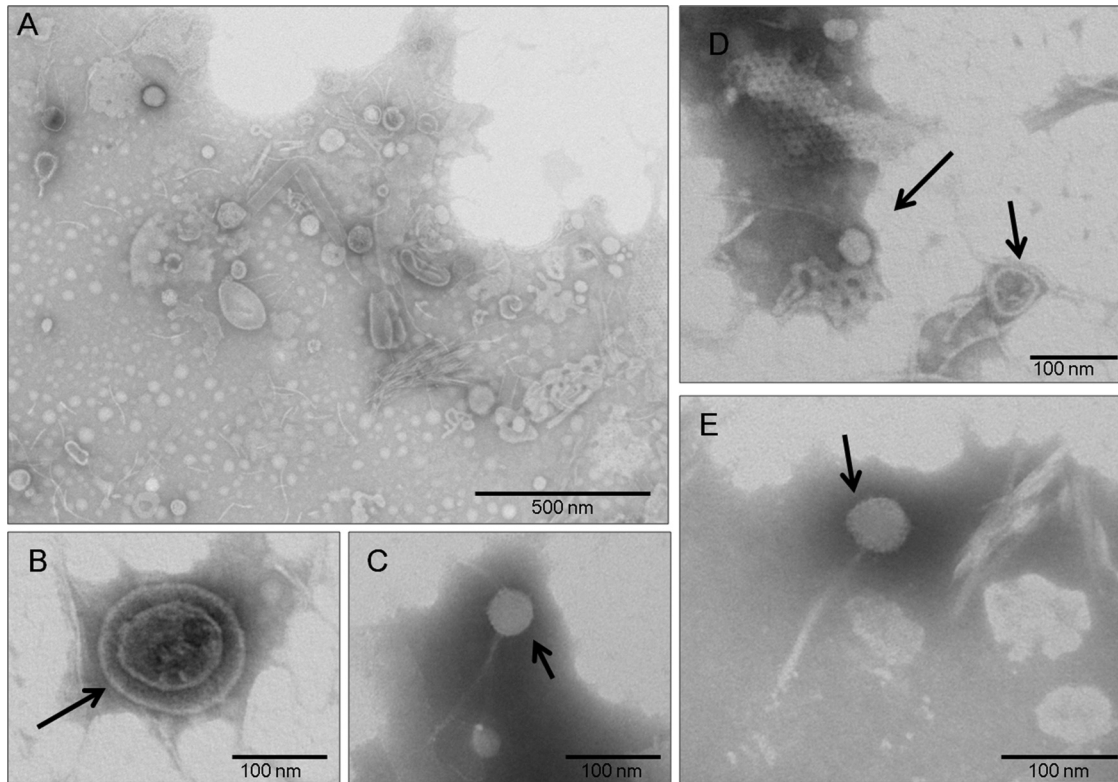
FIG 1 Transmission electron microscopy of negatively stained viral particles. (A) Overview of stained viral particles, which vary in size and shape, isolated from the Middle Ages coprolite. (B to E) A representative virion (B) and virus-like particles (C to E) with icosahedral nucleocapsids and a long filament tail characteristic of Siphoviridae bacteriophages.
