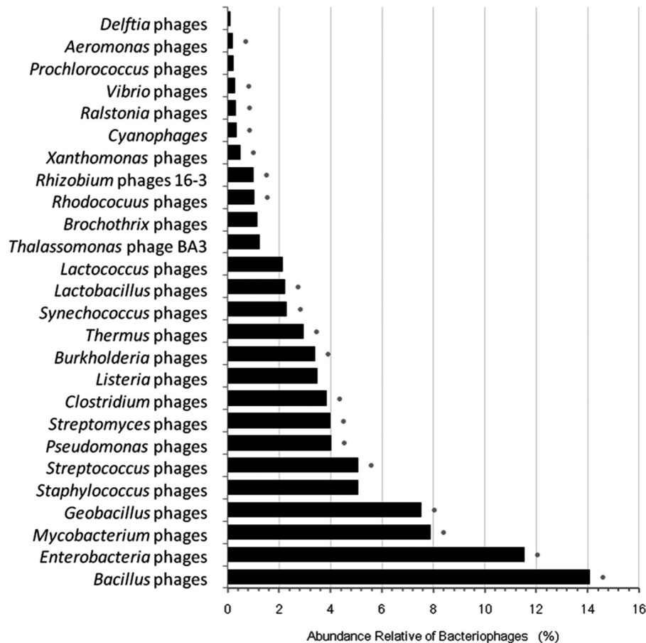
FIG 3 Relative abundance of hits to known bacteriophages. The relative abundance of hits to known bacteriophages was estimated using the GAAS software. The hosts of the bacteriophages that were also identified in a previous study on the bacterial community associated with this specimen (Appelt et al., unpublished data) are noted to the right with dots.
