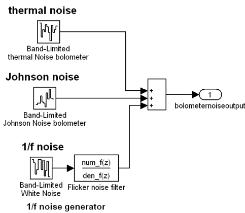
Fig. 3. Noise models associated to the bolometer.
