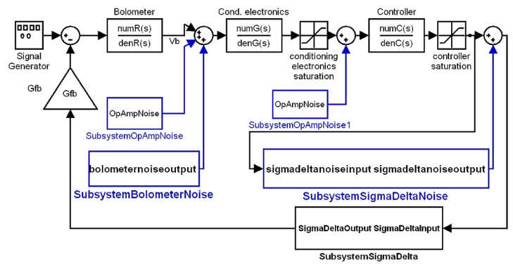
Fig. 7. Diagram of the system.
