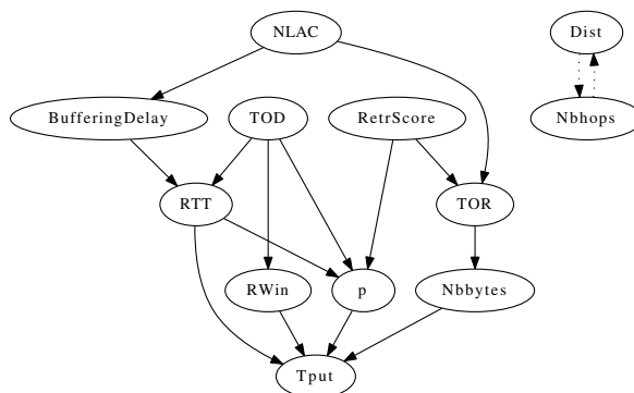
Figure 1: Causal graph model of FTP traffic performance
