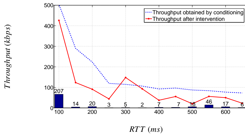
Figure 2: Comparison between causal approach and naive approach
