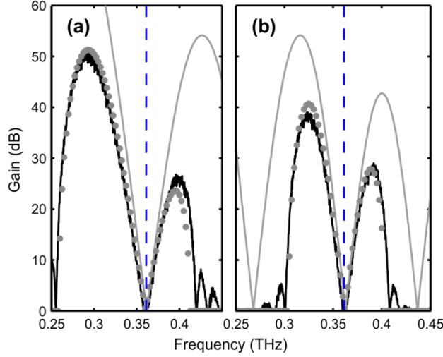
Figure 6 : Output spectrum after 12 kilometers of propagation obtained from numerical simulations (black line), from analytical equation (grey line) and from the Floquet linear stability analysis (grey circles): (a) D_{amp} = 3.7 ps/km/nm; (b) D_{amp} = 6.7 ps/km/nm.
