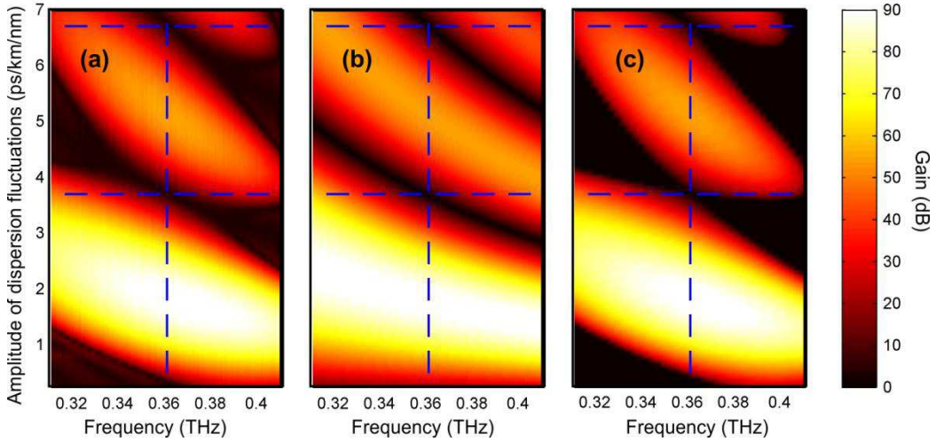
Figure 5 : Magnification of the MI gain spectrum around the first QPM sideband vs. D_{amp} . Numerical results (a) are compared with the analytical results (b) predicted by Eq. (8) and by the Floquet linear stability analysis (c). Blue dashed vertical lines indicates the angular frequency \Omega_l as predicted from Eq. (0) and horizontal lines highlight the values of dispersion fluctuations that are then used in Fig. 6.
