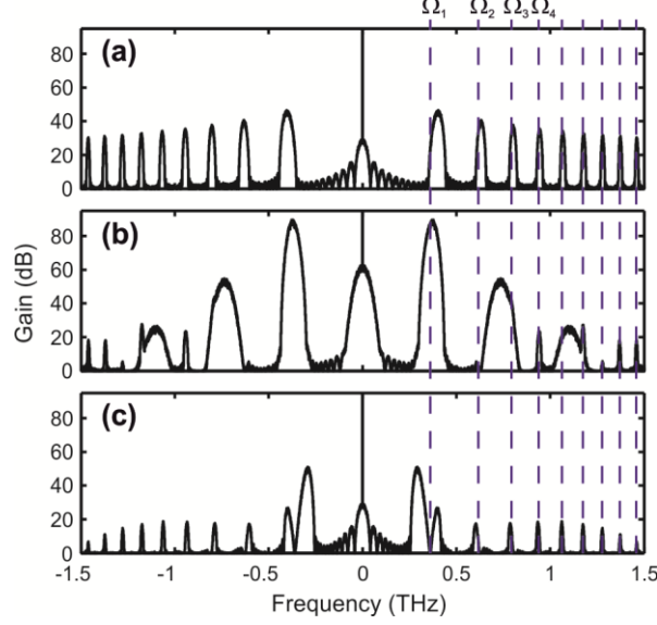
Figure 1 : Evolution of the output spectra recorded after 12 km of propagation for different values of the amplitude of the dispersion fluctuation: D_{amp} = 0.5 ps/km/nm, 1.7 ps/km/nm and 3.7 ps/km/nm, subplots (a), (b) and (c) and respectively. The vertical dashed lines represent the predictions from Eq. (4).
