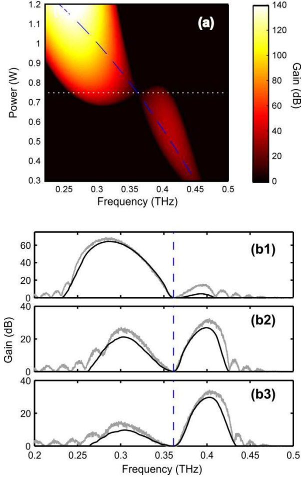
Figure 9 : (a) Evolution of the first sideband after 12 km of propagation according to the input power of the cw and as predicted by the of Floquet linear stability analysis without any loss or gain. The dashed blue line represents the central frequency of the sideband as predicted by Eq. (0), whereas the dotted horizontal line stands for the operating power that has been considered in previous section. (b) Details of the first sideband for the same levels of loss as Fig. 7 : results from numerical integration of Eq. (0) (grey lines) are compared with results from Eq. 9 (black line).
