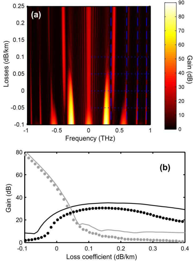
Figure 8 : (a) Evolution of the output spectrum after 12 kilometers of propagation according to the level of linear losses/gain. (b) Evolution of the parametric gain experienced by inner and outer sidebands (grey and black lines or symbols, respectively) according to the level of linear losses/gain. The numerical results (solid lines) are compared with results based on Eq. 9 (dots).
