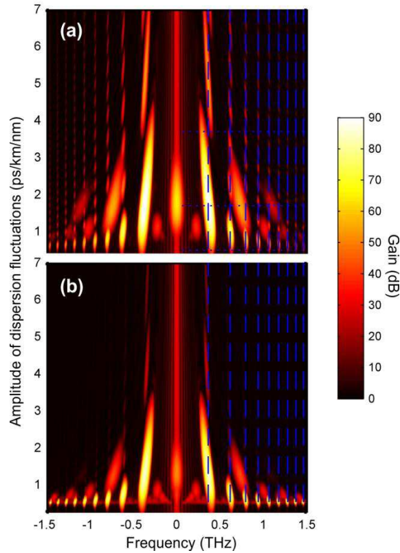
Figure 3 : Evolution of the output MI spectrum after a distance of 12 kilometers according to the level of dispersion fluctuations. (a) Results obtained for a sinusoidal dispersion modulation. (b) Results obtained for a square dispersion modulation. The position of the sidebands predicted from Eq. (0) is plotted with vertical dashed lines. The spectra corresponding to cases of Fig. 1 are highlighted by dashed horizontal lines.
