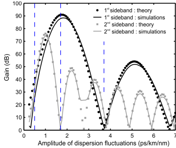
Figure 4 : Evolution with D_{amp} of gain at the frequencies predicted by Eq. (0) for the first and second QPM sidebands (black and grey colors respectively). Results obtained from numerical simulations (solid lines) are compared with analytical predictions from Eq. (0) (circles and squares). Positions of the three cases reported in Fig. 1 are marked with dashed vertical lines.
