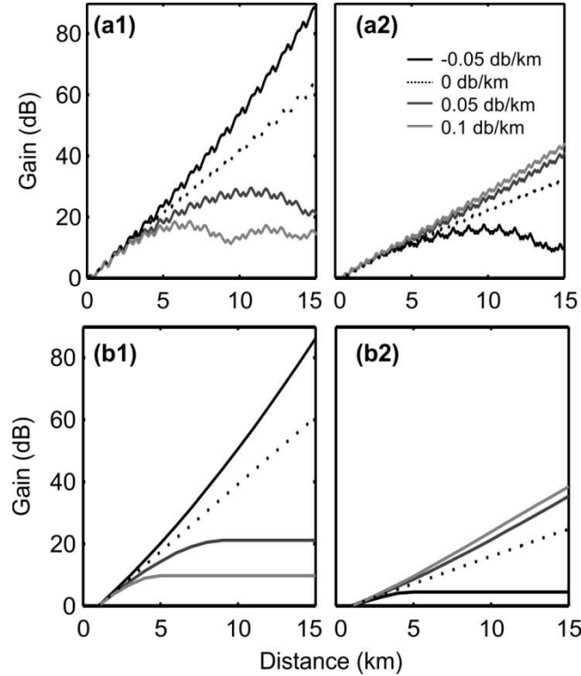
Figure 10 : Longitudinal evolution of the gain for the inner and outer sub-sidebands (panels (a1,b1) and (a2,b2) respectively) for different levels of attenuations/losses: -0.05, 0, 0.05 and 0.1 dB/km, solid black, dotted black, dark grey and light grey lines respectively. Results from numerical simulations (a1,a2) are compared with the results predicted by Eq. 9 (b1,b2).
