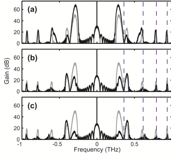
Figure 7 : Evolution of the output spectra after 12 kilometers of propagation for different levels of losses or gain (solid black lines): (a) 0.05 dB/km of gain. (b) 0.05 dB/km of loss. (c) 0.1 dB/km of loss. Results obtained without losses are plotted with grey solid lines.
