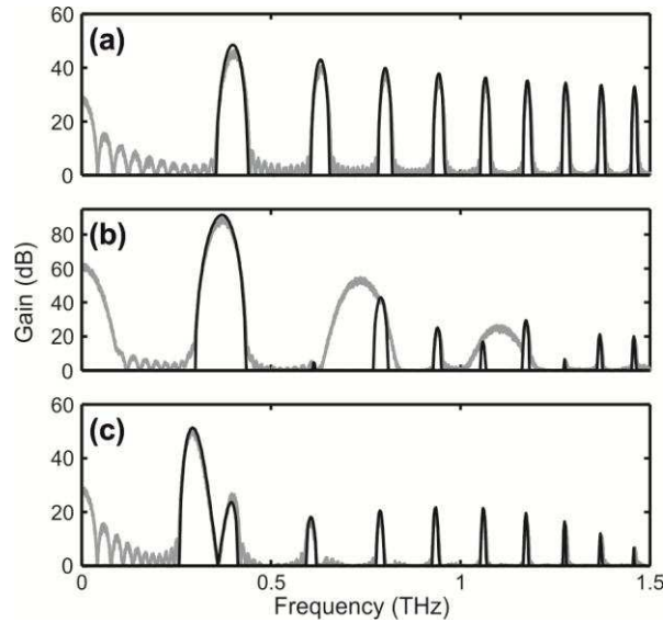
Figure 2 : Anti-Stokes sideband spectrum as Fig.1. The results from the Floquet linear stability analysis of the NLSE with periodic dispersion (black lines) are compared with the results of the numerical integration of Eq. (1) (grey lines)
