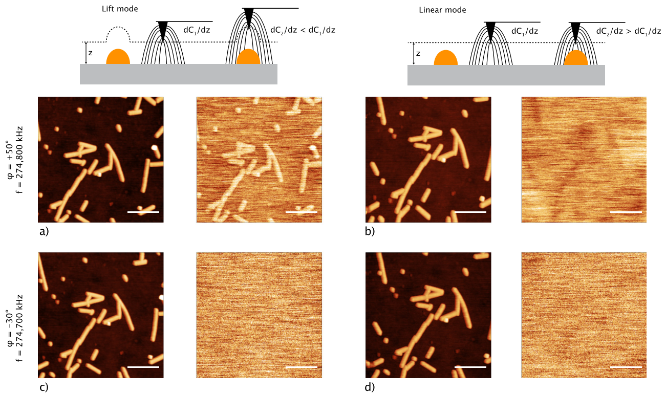
FIG. 9. Topography and KPFM images of tobacco mosaic viruses deposited on silicon dioxide. Scale bars are 500 nm. Colour scales are 25 nm (topography images) and 3 mV (KPFM images). Top: images containing ac cross-talk effects ( \varphi_{\omega} = \varphi_p , see text). Bottom: images free of ac cross-talk effects ( \varphi = \varphi_p \pm 90^\circ , see text). Each couple of images shows the sample topography (left) and the KPFM image (right), acquired with V_{ac} = 2 V, and using a z -offset of 50 nm in the lift or linear modes.
