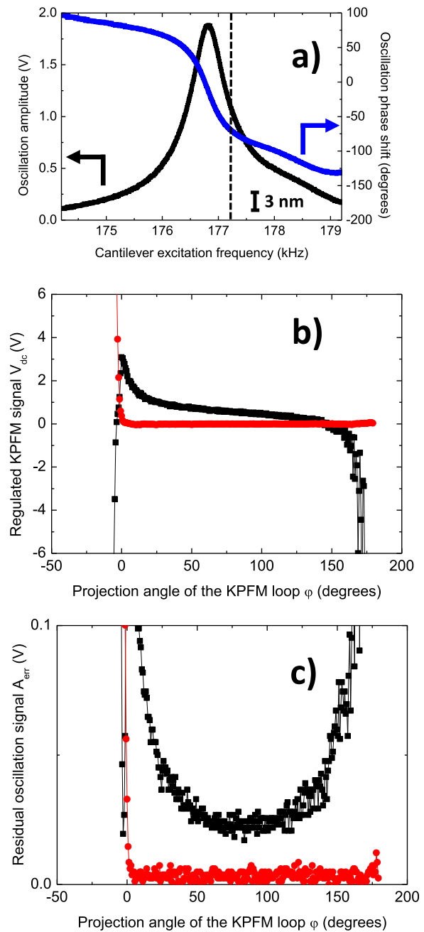
FIG. 4. Same plot as in Figure 3, with the cantilever excited at \omega/2\pi = 177.2 kHz in (b) and (c).
