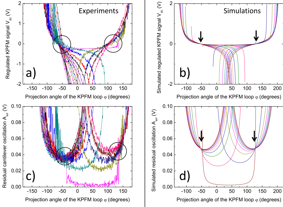
FIG. 6. (a) Experimental values of V_{dc} regulated by the KPFM feedback loop, and plotted as a function of the KPFM feedback loop projection angle \varphi , for the same type of cantilever as in Figs. 3 and 4. Each curve of the plot corresponds to a different excitation frequency or oscillation phase \varphi_\omega across the cantilever resonance (see text). Experimental data have been acquired in presence of the ac cross-talk to the photodiode, only. (b) Simulated values of the V_{dc} potential regulated by the KPFM feedback loop, using the model of Eq. (2) (see text for the details); (c) Experimental values of the residual cantilever oscillation signal A_{err} during the KPFM feedback loop operation. The curves correspond to the V_{dc} data shown in (a); (d) Simulated values of the residual cantilever oscillation signal A_{err} corresponding to the simulated values of V_{dc} in (b).
