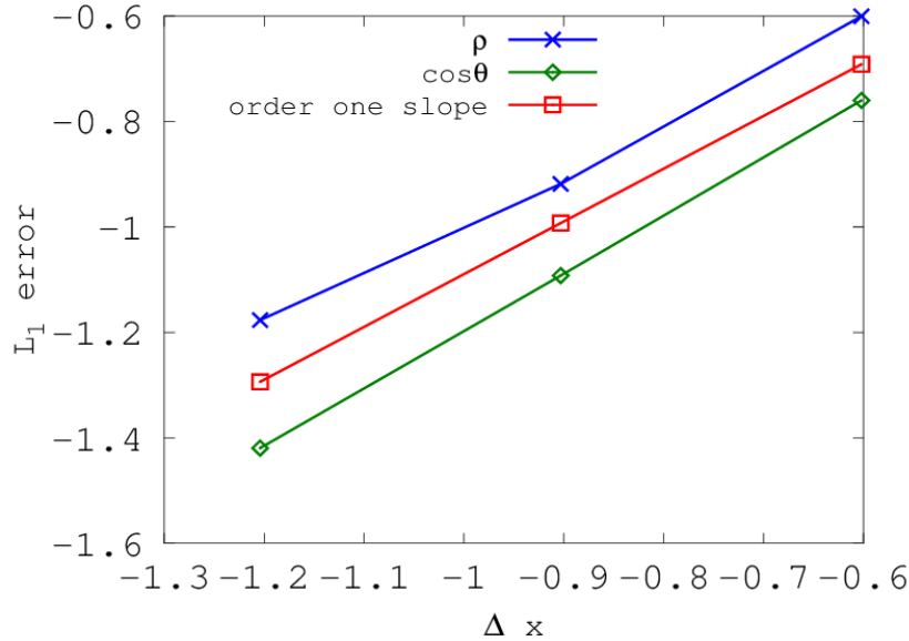
Figure 1: L^1 -error for the density \rho and the flux direction \cos \theta as a function of \Delta x in log-log scale. A straight line of slope 1 is plotted for reference. This figure shows that the scheme is numerically of order 1.
