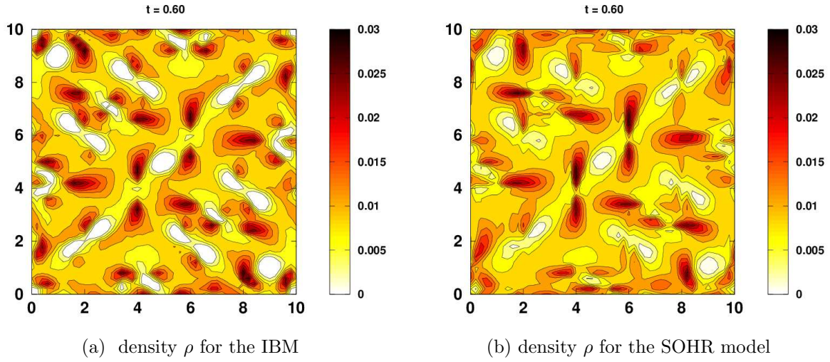
Figure 4: Density \rho for Taylor-Green vortex problem 4.12 at time t = 0.6s . Left: IBM. Right: SOHR model.
