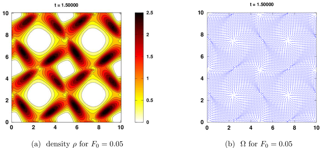
Figure 7: Solution of the SOHR model for F_0 = 0.05 . Density \rho (fig 6a ), flux direction \Omega (fig.6b ) at t = 1.5s .
