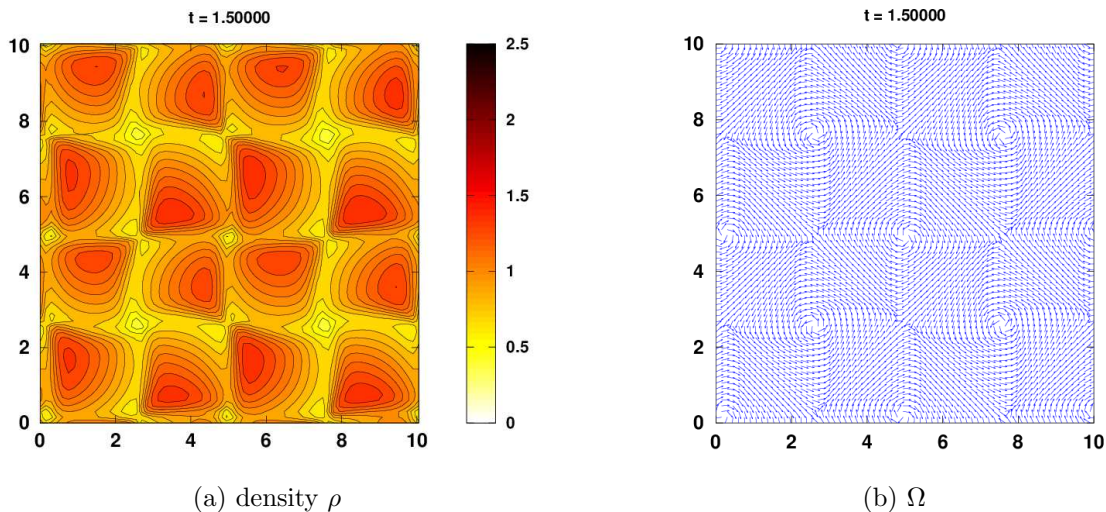
Figure 8: Solution of the DLMP model for F_0 = 5 . Density \rho (left) and flux direction \Omega (right) at t = 1.5s .
