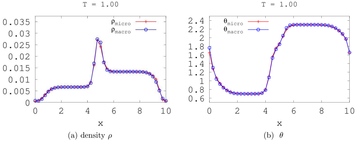
Figure 3: Solution of the Riemann problem (4.11) along the x -axis for the SOHR model (blue line) and for the IBM with \varepsilon = 0.05 (red line) at T = 1s . The agreement between the two models is excellent. For the SOHR model, the mesh size is \Delta x = \Delta y = 0.0625 .
