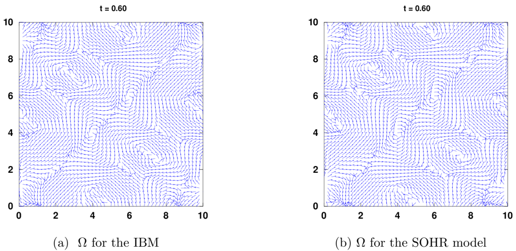
Figure 5: Mean direction \Omega for Taylor-Green vortex problem 4.12 at time t = 0.6s . Left: IBM. Right: SOHR model.
