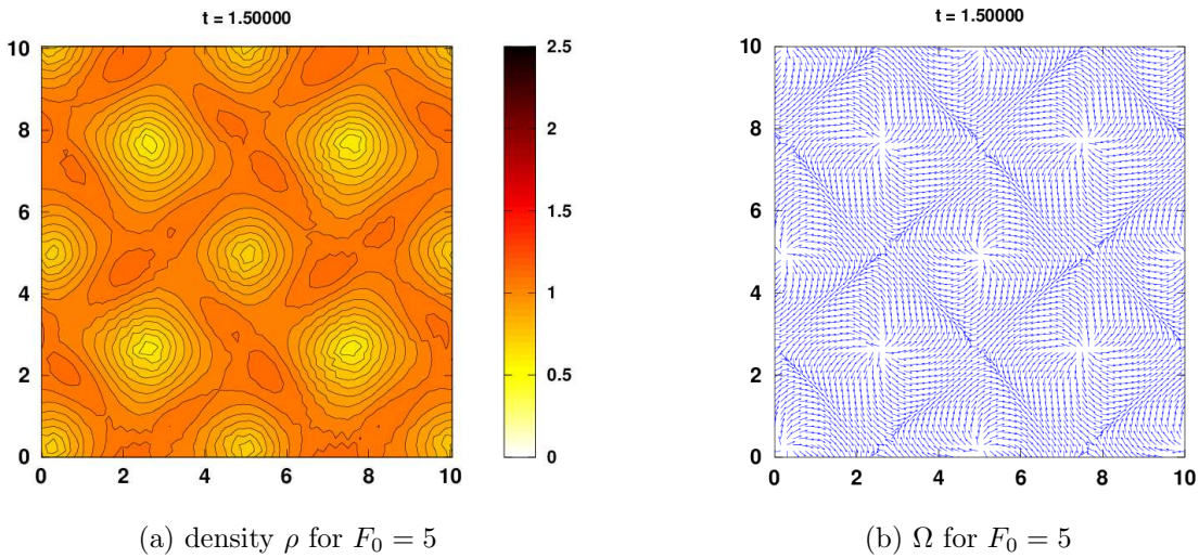
Figure 6: Solution of the SOHR model for F_0 = 5 . Density \rho (fig 6a ), flux direction \Omega (fig.6b ) at t = 1.5s .
