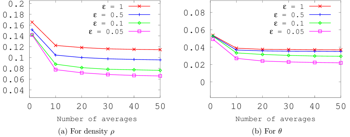
Figure 2: Relative error between the macroscopic and the microscopic model for density (a) and \theta (b) as a function of the number of averages for different values of \varepsilon . The error decreases with both decreasing \varepsilon and increasing number of averages, showing that the SOHR model provides a valid approximation of the IBM for \rho and \theta .
