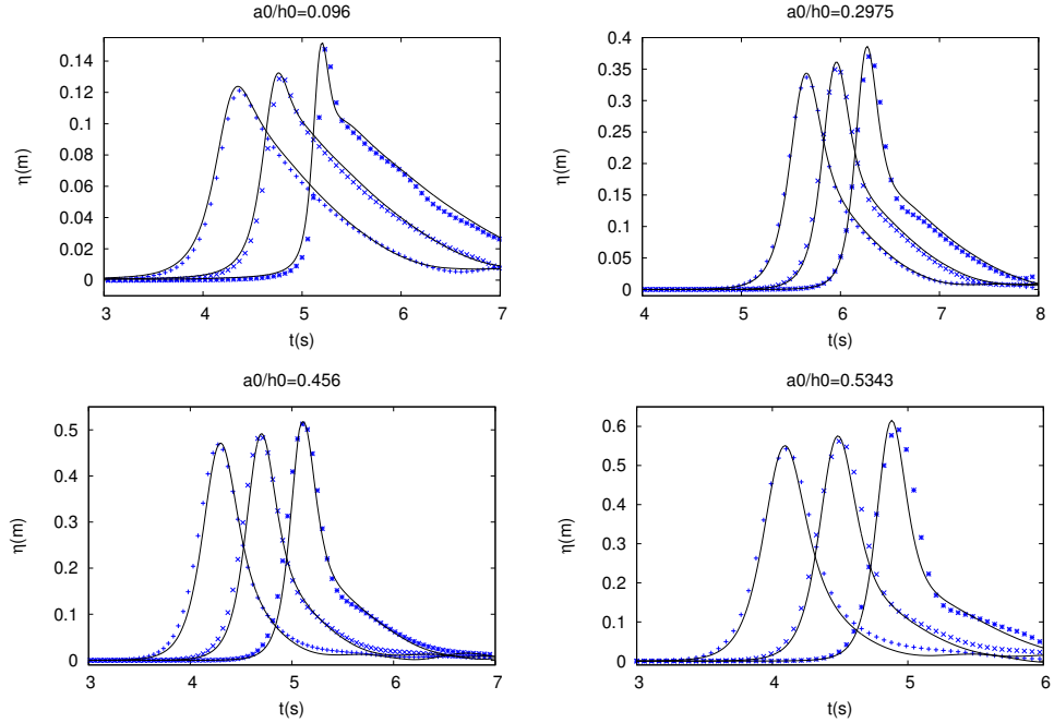
Figure 11: Guibourg test case : comparison between computed (solid lines) and experimental (dots) time series of total free surface at several gauges before the breaking point.
