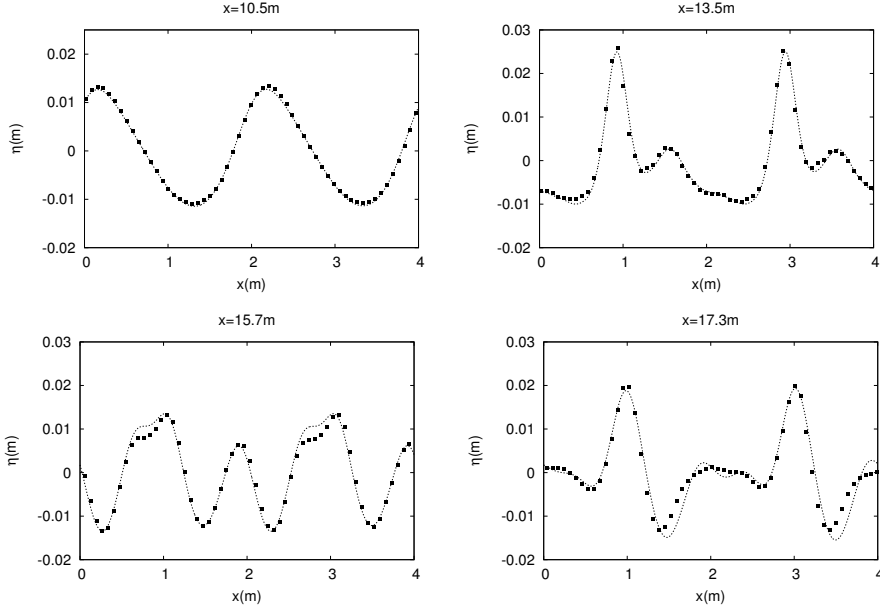
FIGURE 10. Propagation of highly dispersive waves : free surface evolution at the four first gauges. Experimental data are denoted by squares.
