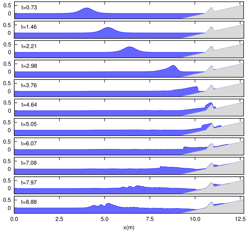
FIGURE 16. Overtopping over fringing reefs : Free surface profiles at several times during the propagation.
