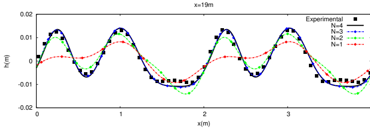
FIGURE 11. Propagation of highly dispersive waves : several profiles for increasing N at the last gauge.
