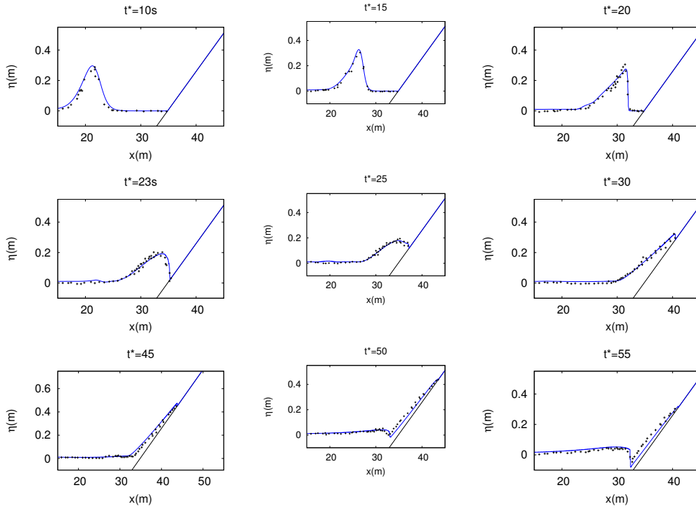
FIGURE 12. Solitary wave breaking over a sloping beach : free surface profiles comparison between numerical results (solid lines) and experimental data (dots) at several times during the breaking ; t^* = t(g/h_0)^{1/2} .
