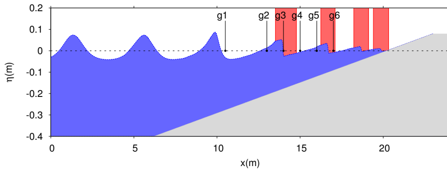
FIGURE 13. Cox's experiment : sketch of the basin and identification of breaking areas. The NSW equations are used in red areas to describe the breaking waves.
