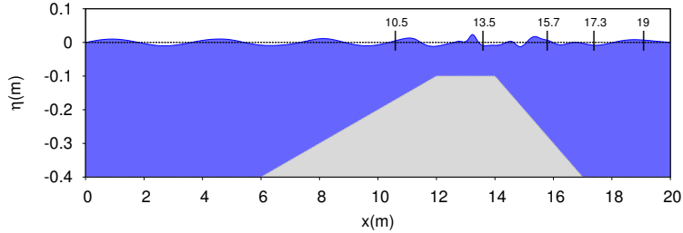
FIGURE 9. Periodic waves over a submerged bar : sketch of the basin and gauges location.
