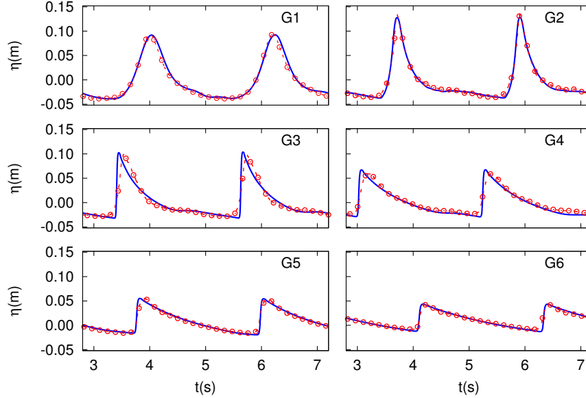
FIGURE 14. Cox’s experiment : comparison between computed and experimental time series of total free surface at the gauges.
