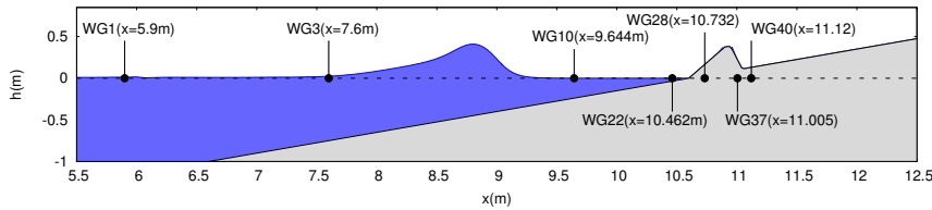
FIGURE 15. Overtopping over fringing reefs : sketch of the basin and gauge locations.
