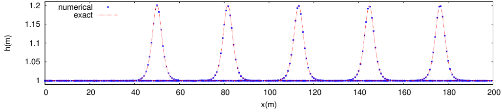
FIGURE 7. Propagation of a solitary wave : water surface profiles at t=0.4, 0.8, 1.2, 1.6 and 2s .
