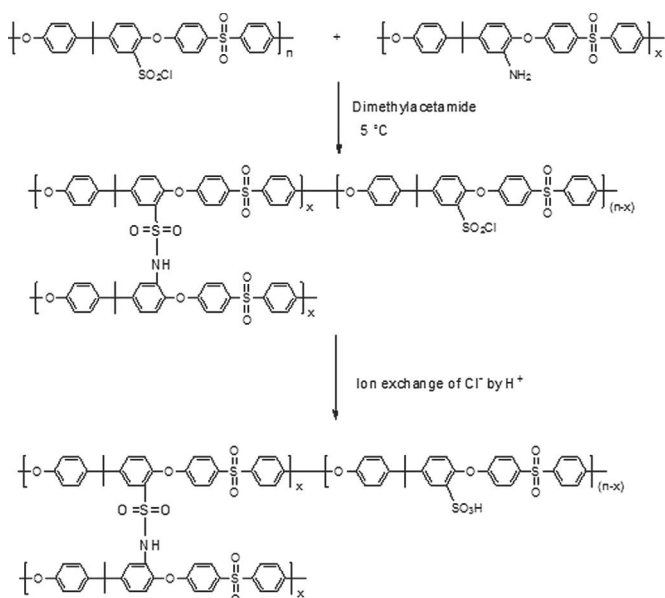
Fig. 2. Scheme of crosslinking of \text{CINH}_2 membranes.
