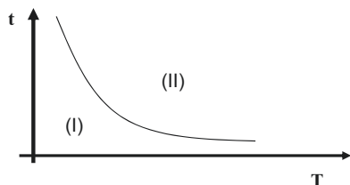
Fig. 1. Schematization of the stability domain of POOH groups in the time-temperature space; hydroperoxides are stable in domain (I).
