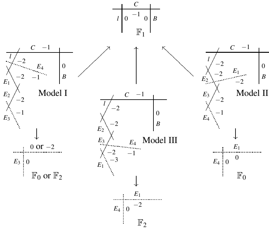
FIGURE 7. The three models of pencils with their resolution (the index of the exceptional divisors E_i corresponds to their order of construction coming from \mathbb{F}_1 ).
