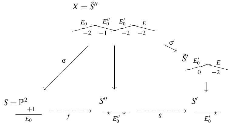
FIGURE 4. The counter-example in Remark 8 (* denotes a singularity, numbers are self-intersections)
