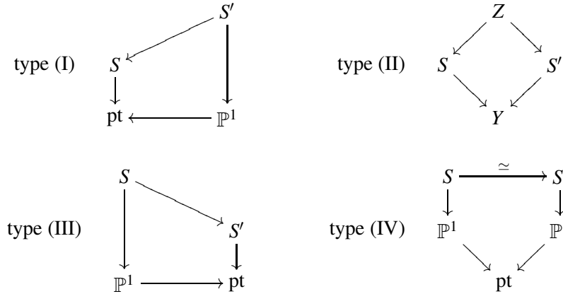
FIGURE 1. The four types of links of the log Sarkisov program.
