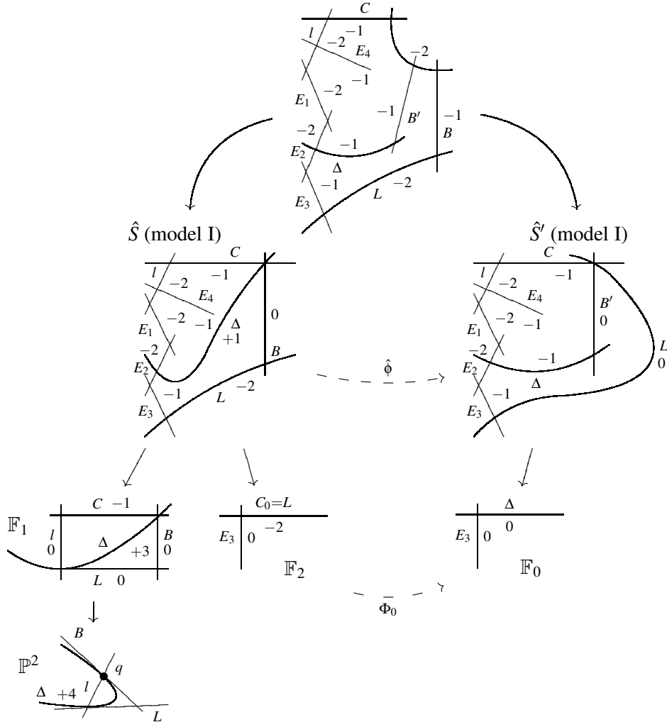
FIGURE 8. Quadratic triangular map \Phi_0: (\mathbb{F}_2, D_2) \dashrightarrow (\mathbb{F}_0, D_0) .
