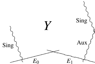
FIGURE 3. The boundary divisor of Y .
