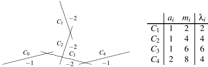
FIGURE 2. Resolution of f and coefficients in the ramification formulas.
