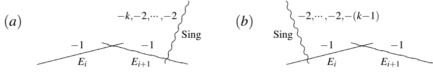
FIGURE 5. Boundary of Y in the proof of Lemma 12.
