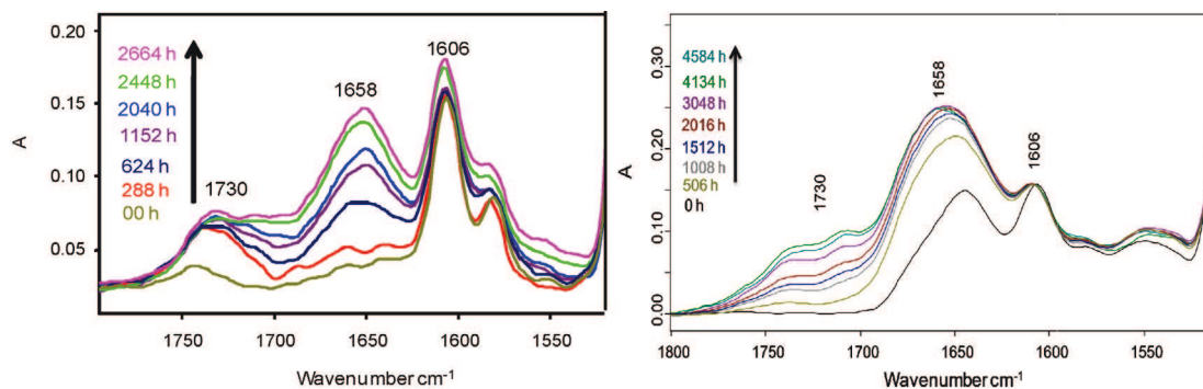
Fig. 3. FTIR spectra in the 1520–1800 \text{cm}^{-1} domain, left: POPA system, right: PAA system during exposure in air at 110 °C.
