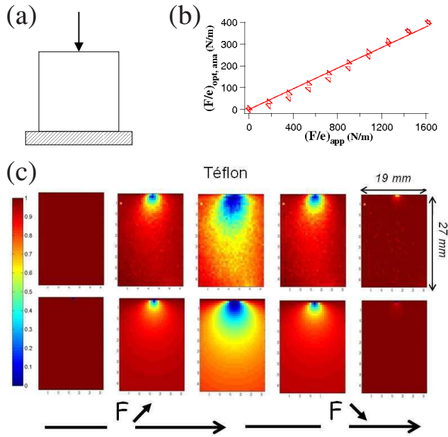
Fig. 3. Point load configuration, (a) the load is applied with a blade, a null displacement is imposed at the opposite side of the sample ; (b) comparison of the force applied experimentally divided by the thickness of the sample with the value obtained by the best fit with eq. 6. The slope of the linear fit is 0.24 ; (c) upper line : experimental decorrelation maps ; bottom line : best analytical fit with eq. 6
