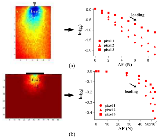
Fig. 5. Examples of correlation maps g_I(x, z) obtained for Teflon (a) and granular (b) samples for given values of \Delta F . The position and size of the tips are indicated on top of the images. For the three pixels indicated on each map, we plot \ln(g_I)_{\text{pixel}} as a function of the force increment \Delta F during the first loading.
