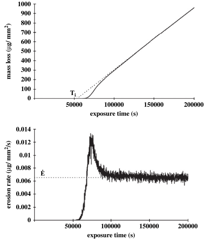
Fig. 6. (a) Mass loss (up) and (b) erosion rate (down) calculated as a function of the exposure time. Simulations are based on Al234 pitting test (Table 2). The value of the incubation time T_i is obtained from (a) as indicated in the figure. The steady-state erosion rate \dot{E} is obtained from (b). The value of the volumic erosion rate V_{er} is calculated from \dot{E} = \rho V_{er} (see Eq. (19)).
