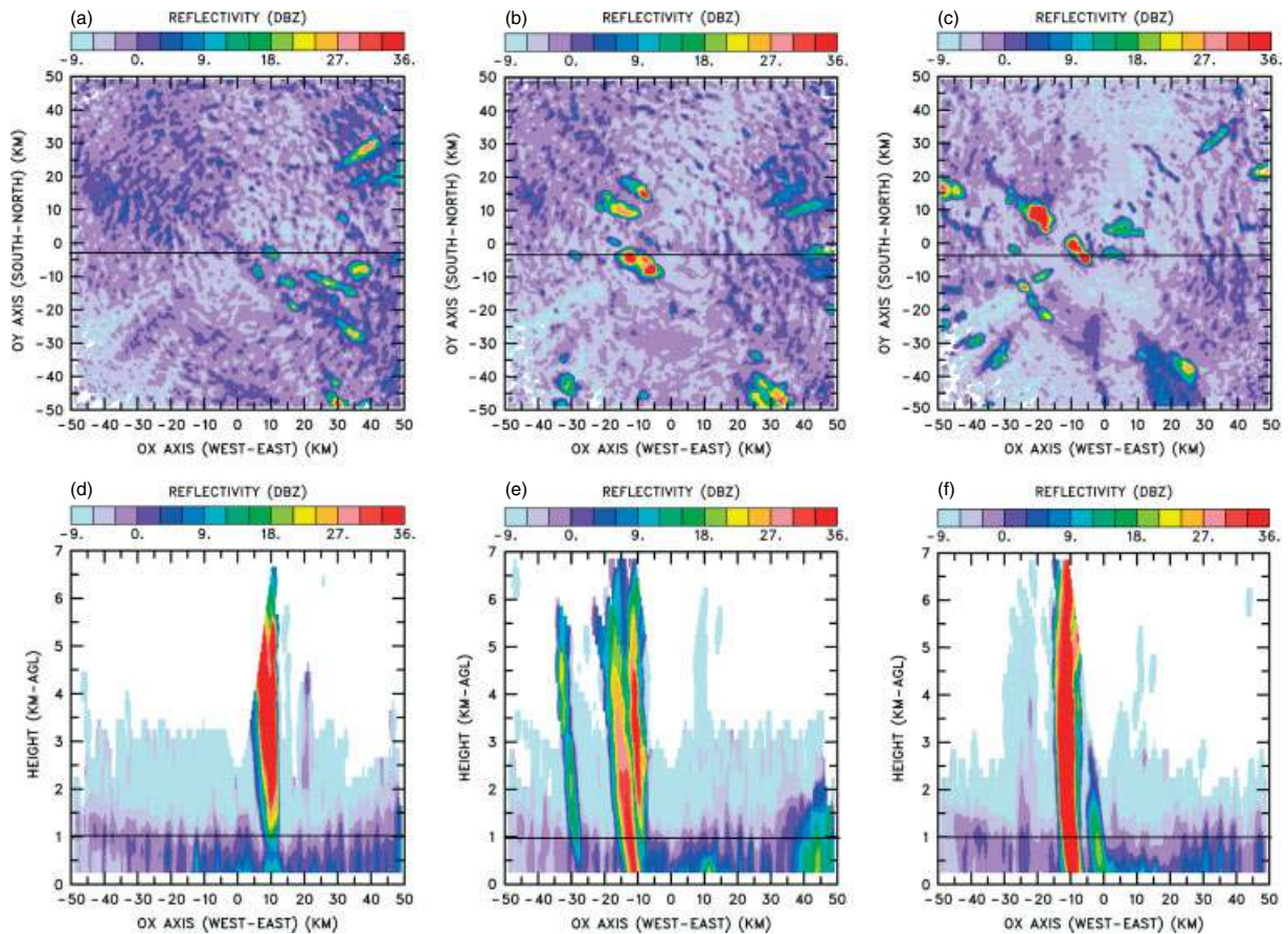
Figure 3. Reflectivity interpolated onto (a, b, c) horizontal cross-sections at Z = 1000 m agl, and (d, e, f) vertical cross-sections at Y = -3 km, at (a, d) 1510 UTC, (b, e) 1600 UTC, and (c, f) 1700 UTC on 27 July 2006. The MIT radar was positioned at the reference point ( X = 0 , Y = 0 ). Here R_{xy} = 1000 m and R_z = 500 m are used for the horizontal and vertical sections. Straight lines indicate positions of the vertical and horizontal cross-sections shown. High reflectivity in the southeast sector ( X = 30 km, Y = 0 km) at 1600 UTC are second-trip echoes from long-distance deep convective systems.
