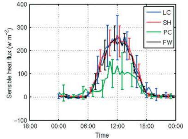
Figure 9. Composite diurnal cycle of sensible heat flux from the surface flux data at Niamey Airport, for each class. Error bars represent the standard deviation over the cases in the class.
