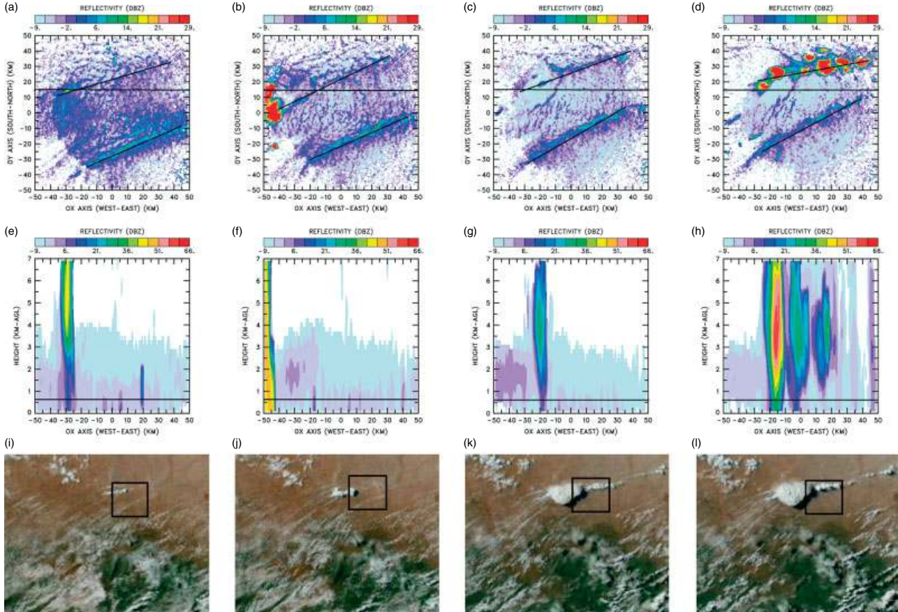
Figure 5. Reflectivity on 6 July 2006 interpolated onto (a, b, c, d) horizontal cross-sections at Z = 600 m agl, (e, f, g, h) vertical cross-sections at Y = 15 km, at (a, e) 1500 UTC, (b, f) 1550 UTC, (c, g) 1620 UTC, and (d, h) 1640 UTC. Here R_{xy} = 600 m and R_z = 350 m are used for the horizontal sections and R_{xy} = 1000 m and R_z = 1000 m for the vertical sections. Horizontal straight lines indicate the positions of the vertical and horizontal cross-sections. In (a, b, c, d), the diagonal black lines indicate the orientation of observed convergence lines. (i, j, k, l) show satellite visible cloud images at 1500, 1530, 1630 and 1645 UTC respectively, with the square indicating the scan volume ( 100 \text{ km} \times 100 \text{ km} ) of the MIT radar.
