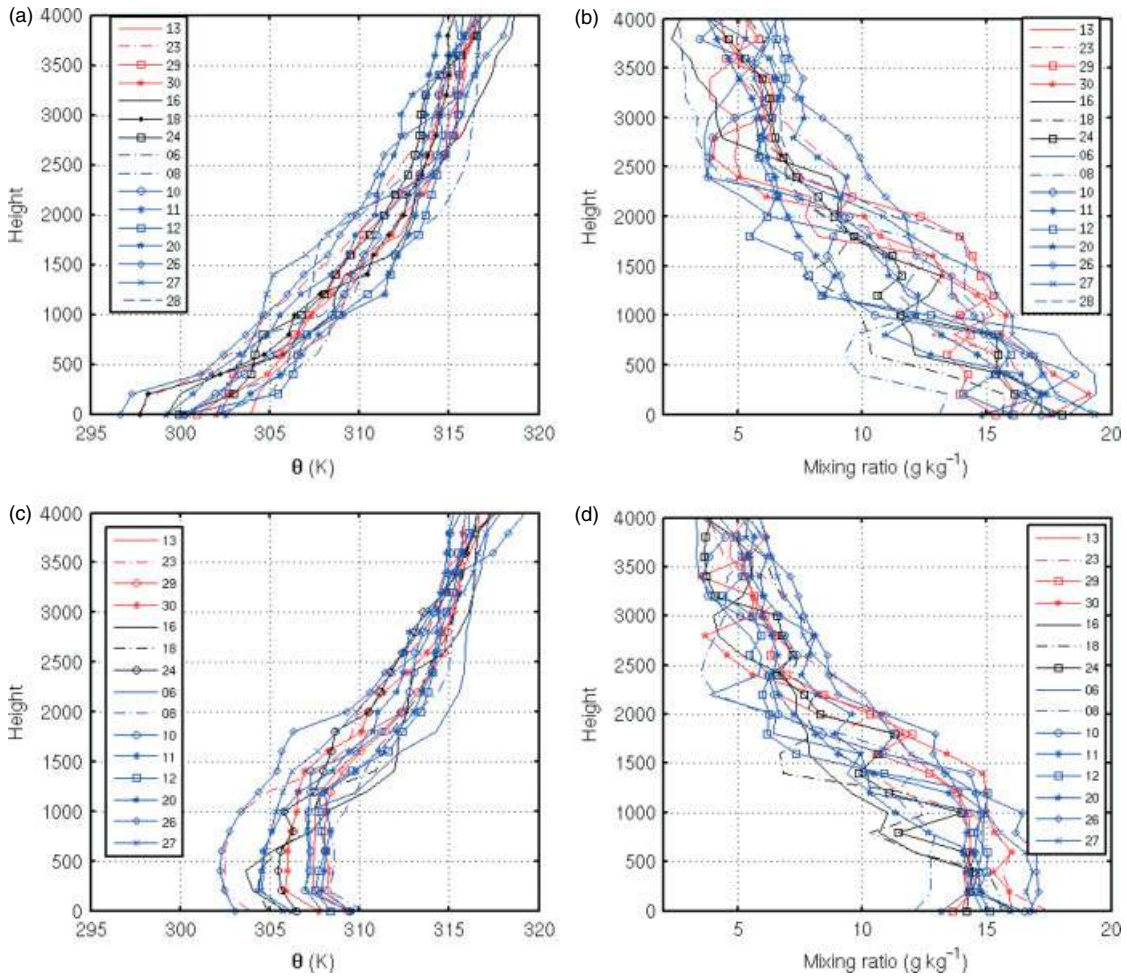
Figure 10. Vertical profiles of (a, c) potential temperature \theta and (b, d) mixing ratio at (a, b) 0530 UTC and (c, d) 1130 UTC on each day with the assigned class shown: shallow convection (red), fair weather (black) and locally initiated deep convection (blue).
