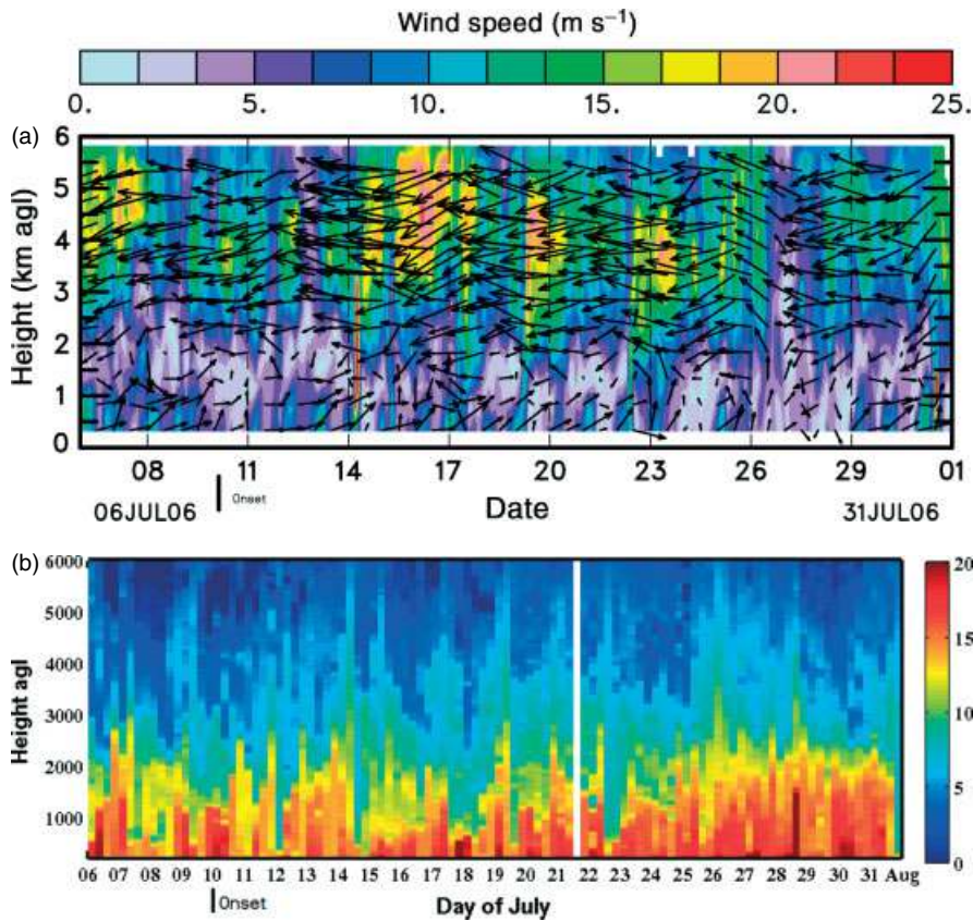
Figure 2. Time–height section of (a) the horizontal wind ( \text{m s}^{-1} ) measured with the UHF wind profiler and (b) mixing ratio ( \text{g kg}^{-1} ) measured by the radiosondes at Niamey from 6 to 31 July 2006. In (a), a leftward arrow represents an easterly wind.
