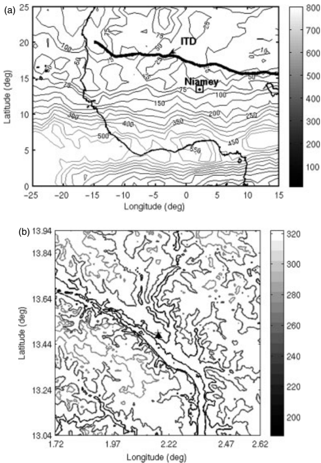
Figure 1. (a) Total rainfall (mm, greyscale contours) for July 2006 in West Africa from the Global Precipitation Climatology Project (GPCP). The thick black line indicates the averaged position of the ITD in July (line of constant dewpoint temperature at 2 m, equal to 15°C). The small square indicates the study area. (b) shows the topography (m) within this study area, with the location of the MIT radar (+) and the ARM site (with radiosonde, UHF wind profiler, and the 95 GHz cloud radar) (▲).
