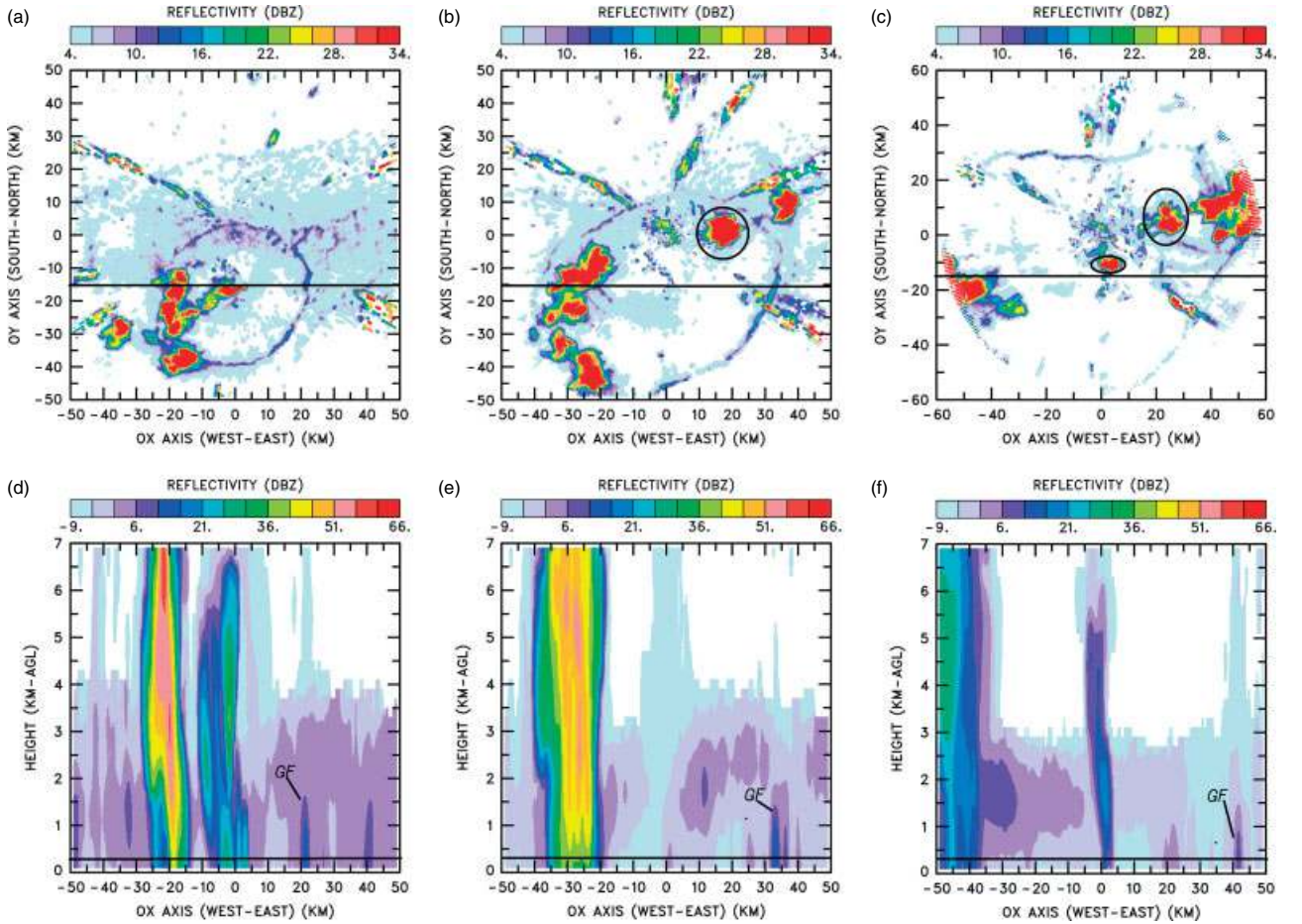
Figure 6. Reflectivity interpolated onto (a, b, c) horizontal cross-sections at Z = 300 m agl, and (d, e, f) vertical cross-sections at Y = -15 km, at (a, d) 1610 UTC, (b, e) 1640 UTC, and (c, f) 1730 UTC on 11 July 2006. The MIT radar was positioned at the reference point ( X = 0 , Y = 0 ). Here R_{xy} = 600 m and R_z = 350 m are used for interpolation on the horizontal sections and R_{xy} = 1000 m and R_z = 1000 m for the vertical sections. Cells triggered by the gust front are circled in black. ‘GF’ indicates the top of the gust front. In (a, b, c) a minimum radar reflectivity of 4 dBZ on the colourscale is used to mask the clear air organisation and to point out the clear signature of the gust front.
