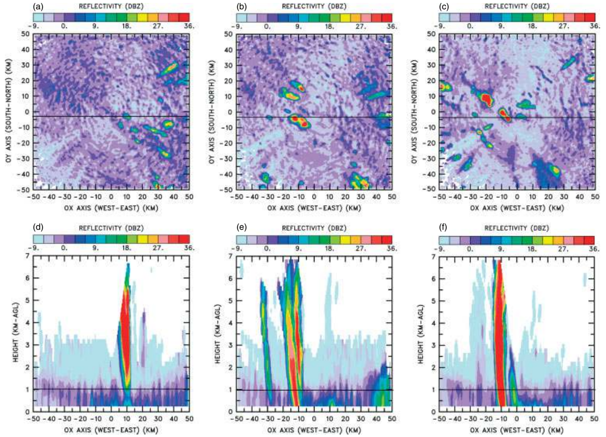
Figure 3. Reflectivity interpolated onto (a, b, c) horizontal cross-sections at Z = 1000 m agl, and (d, e, f) vertical cross-sections at Y = -3 km, at (a, d) 1510 UTC, (b, e) 1600 UTC, and (c, f) 1700 UTC on 27 July 2006. The MIT radar was positioned at the reference point ( X = 0 , Y = 0 ). Here R_{xy} = 1000 m and R_z = 500 m are used for the horizontal and vertical sections. Straight lines indicate positions of the vertical and horizontal cross-sections shown. High reflectivity in the southeast sector ( X = 30 km, Y = 0 km) at 1600 UTC are second-trip echoes from long-distance deep convective systems.
