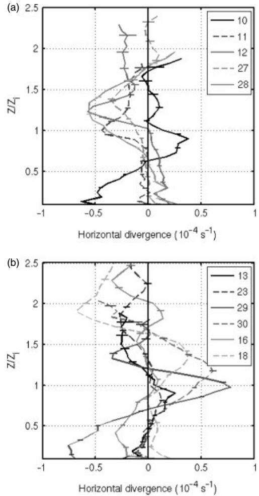
Figure 12. Horizontal divergence averaged between 1100 and 1500 UTC as a function of normalised height: (a) afternoon local deep convection days, (b) shallow convection days (13, 23, 29, and 30) and fair weather days (16 and 18).
