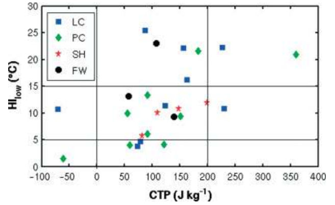
Figure 8. CTP and HI_{low} at 0530 UTC. Classes are as in Figure 7.
