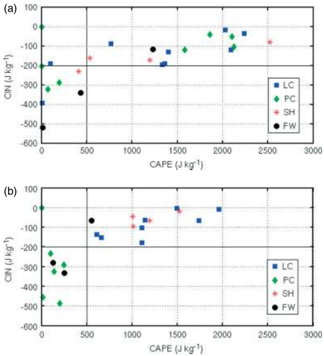
Figure 7. CIN as a function of CAPE at (a) 0530 UTC and (b) 1130 UTC for all days from 6 to 31 July 2006. LC are cases of locally initiated deep convection, PC cases of propagating deep convection, SH cases of shallow convection and FW cases of fair weather. Note that the radiosonde on 28 July at 1130 UTC is erroneous, and is not shown here.
