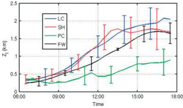
Figure 11. Composite diurnal cycle of the CBL height for each class deduced from the UHF wind profiler: afternoon local deep convection days (blue), shallow convection days (red), propagating deep convection days (green) and fair weather days (black). We considered that the boundary-layer depth is not defined during a rainfall event.
