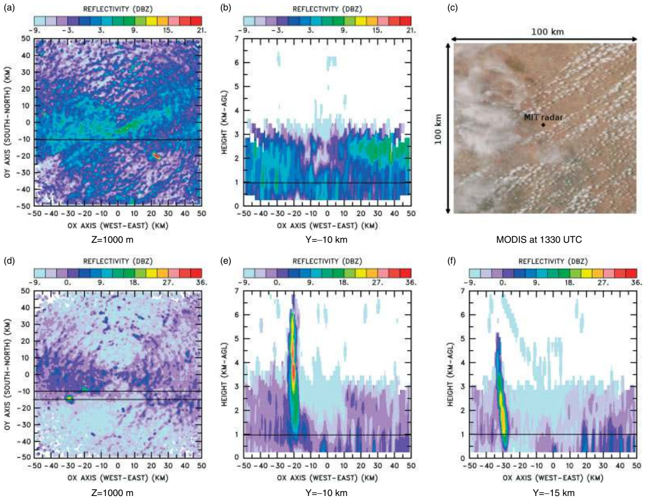
Figure 4. Example of a shallow convection case, on 13 July 2006, at (a, b, c) 1330 UTC and (d, e, f) 1640 UTC. MIT radar interpolated reflectivity (with influence radii as in Figure 3) onto (a, d) horizontal cross-sections at Z = 1000 m, and (b, e, f) vertical cross-sections south of the radar – (b, e) at Y = -10 km and (f) at Y = -15 km. Straight lines indicate the vertical and horizontal cross-sections shown. Colour scales are different between (a, b) and (d, e, f) because in (a, b) low reflectivity is chosen for the observation of the clear air organisation.
