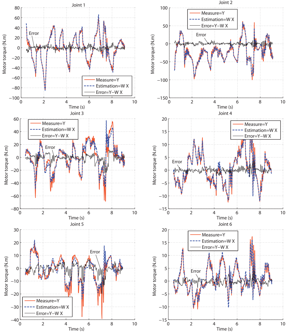
Fig. 2. Motor torques (joint side units) calculated with identified gains (red) and with IDIM (blue) of the TX-40 with the payload of 4.59kg.
