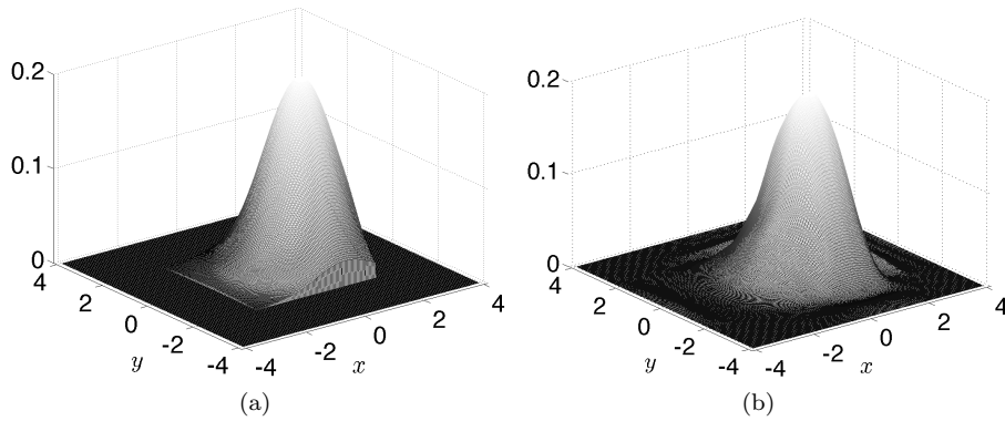
Fig. 1 (a) Theoretical density h . (b) Block thresholding estimator \hat{h} from a single simulation.
