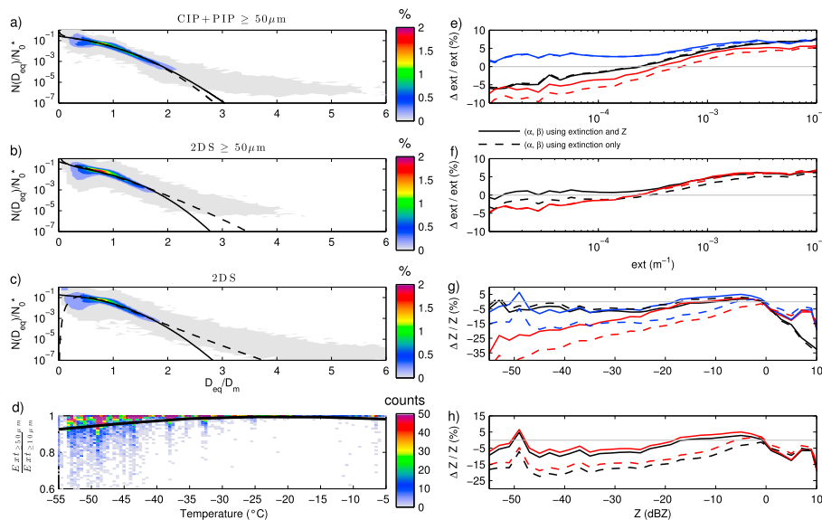
Figure A2. Impact of the small particle contribution on the normalized PSD shape. (a–c) The normalized PSD shapes for CIP+PIP data, 2D-S data when particles below 50 μm are removed and all 2D-S data, respectively. (d) The ratio of extinction derived using 2D-S data without small particles to extinction derived using all 2D-S data as a function of cloud temperature. (e–h) Relative differences (in percent) obtained with or without removing small particles. Details are in the text.
