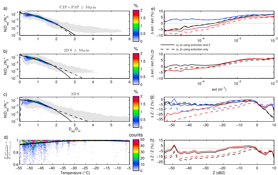
Figure A2. Impact of the small particle contribution on the normalized PSD shape. (a–c) The normalized PSD shapes for CIP+PIP data, 2D-S data when particles below 50 \mu\text{m} are removed and all 2D-S data, respectively. (d) The ratio of extinction derived using 2D-S data without small particles to extinction derived using all 2D-S data as a function of cloud temperature. (e–h) Relative differences (in percent) obtained with or without removing small particles. Details are in the text.
