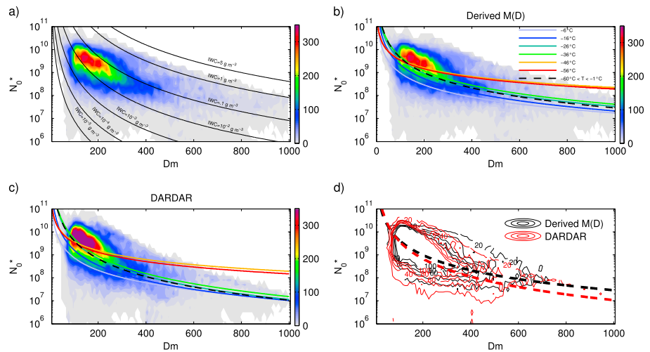
Figure 15. N_0^* - D_m relationships. (a) A PDF of N_0^* ( m^{-4} ) as a function of D_m (micron) computed using the measured PSD and retrieved M(D) . Black lines represent N_0^* - D_m relationships at constant IWC. (b) Identical to Figure 15a but including fits for each temperature range. (c) The same as Figure 15b assuming DARDAR M(D) . (d) Parameterizations obtained for the full range of temperature for the retrieved and DARDAR M(D) are compared. Isocontours represent the number of data.
