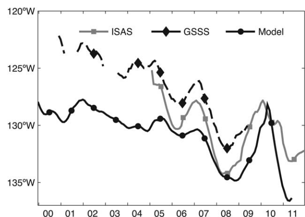
Figure 8. Interannual variability of the longitudinal location of the barycenter of high-salinity ( S > 36 pss) waters based on the model (black dots), the VOS-derived (black diamonds) and ARGO-derived (gray squares) gridded SSS product data sets. Barycenter locations are shown for the observations only when at least half of the data within the east-box is above the error criterion described in section 2.
